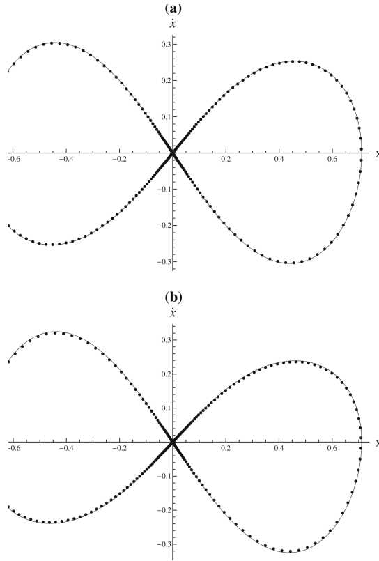
Figure 1: Figure 1. (Original Fig. 1) Homoclinic orbits for \varepsilon = 1.2, 2.0 . Solid lines: Runge–Kutta method. Dotted lines: GHFP method. Excellent agreement demonstrates the effectiveness of the quadratic generalized harmonic function approach for rational restoring forces.
