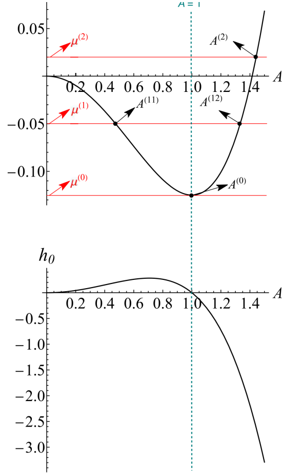
Figure 2: Figure 1. (Upper) Relationship between limit cycle amplitude A and control parameter \mu_c . (Lower) Characteristic quantity h_0 determining stability. Key bifurcation points: \mu^{(0)} = -0.1249 (semi-stable cycle emerges), \mu^{(1)} = -0.05 (splits into stable + unstable), \mu^{(2)} = 0.02 (unstable cycle collapses to singular point).
