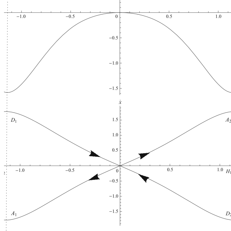
Figure 5: Potential energy curve and homoclinic orbits of the SD oscillator (112) with double-well structure. The two homoclinic orbits around different saddles are both accurately captured.
