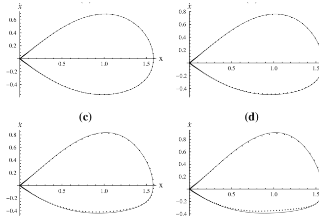
Fig. 2 Homoclinic orbit of oscillator (65) for a \varepsilon = 0.5 , b \varepsilon = 1.0 , (c) \varepsilon = 1.5 and (d) \varepsilon = 2.0 . Continue denotes the orbits obtained by Runge–Kutta method; dotted line denotes the orbits obtained by present method
