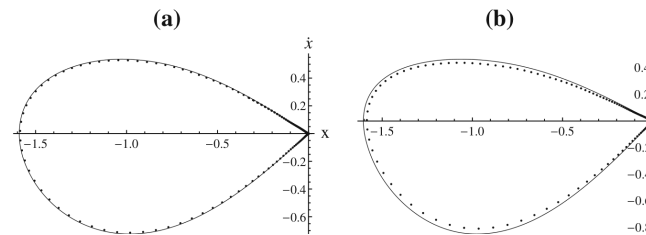
Figure 2: Figure 2. (Original Fig. 2) Homoclinic orbits for \varepsilon = 0.5, 1.0, 1.5, 2.0 . The method successfully tracks the orbits across a wide range, maintaining accuracy even at \varepsilon = 2.0 .
