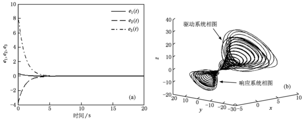
Figure 2: (a) Synchronization error curves for \alpha = -2 ; (b) three-dimensional GPS phase portraits of drive and response systems for \alpha = -2 . The response phase portrait is an anti-phase compressed replica of the drive.
