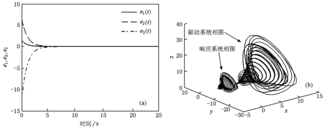
Figure 3: (a) Synchronization error curves for \alpha = 3 ; (b) three-dimensional GPS phase portraits for \alpha = 3 , showing in-phase compression.
