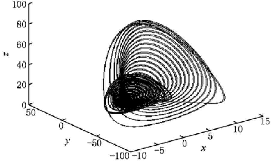
Figure 1: Three-dimensional chaotic phase portrait of the energy resource system Eq. (8).
