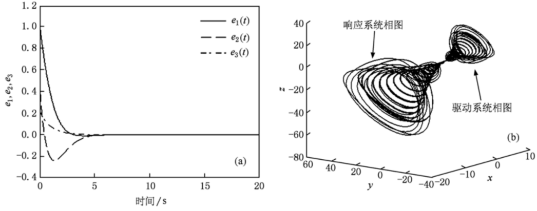
Figure 4: (a) Heterostructure synchronization error for \alpha = -0.5 (anti-phase stretch); (b) three-dimensional GPS phase portraits for \alpha = -0.5 .
