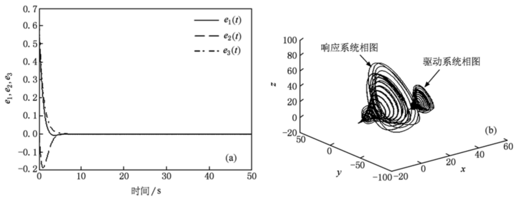
Figure 5: (a) Heterostructure synchronization error for \alpha = 0.4 (in-phase stretch); (b) three-dimensional GPS phase portraits for \alpha = 0.4 .
