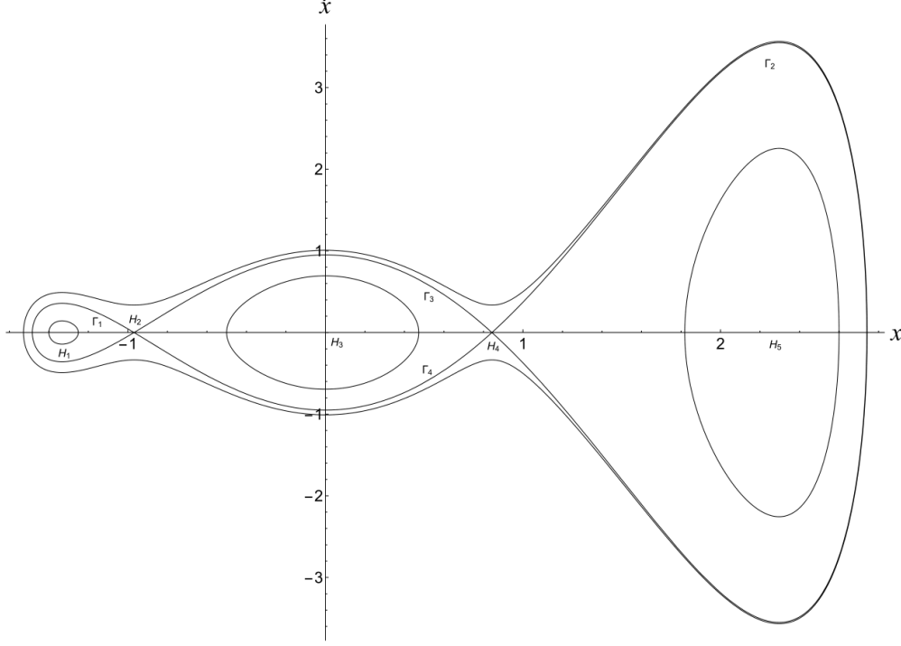
Figure 1: Phase portraits of the \Phi^6 -Van der Pol oscillator with asymmetric potential. GPLP accurately captures both homoclinic orbits despite the asymmetry.
