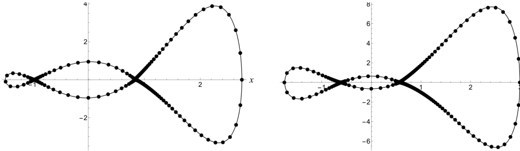
Figure 2: Homo-heteroclinic orbits of the DH-VDP oscillator. The method maintains accuracy at \varepsilon = 1 .
