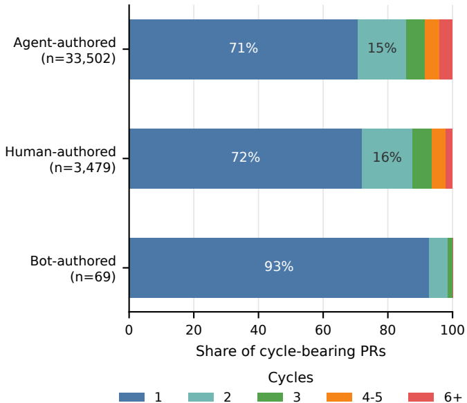
A. Cycles per cycle-bearing PR
