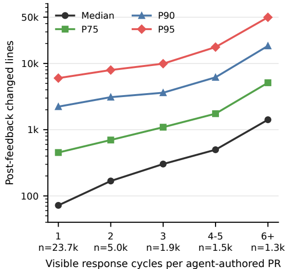
B. Agent revisions by cycle count
