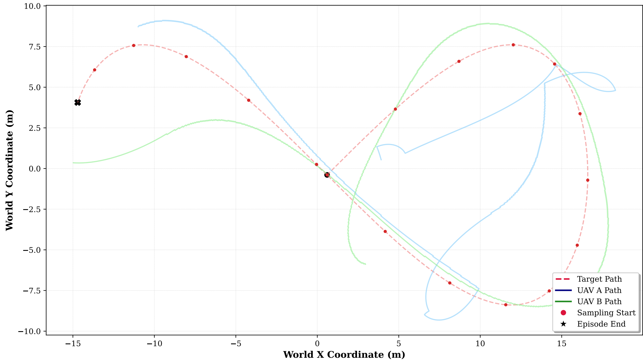
Hierarchical Trajectory Dataset Analysis (Episode 6)
