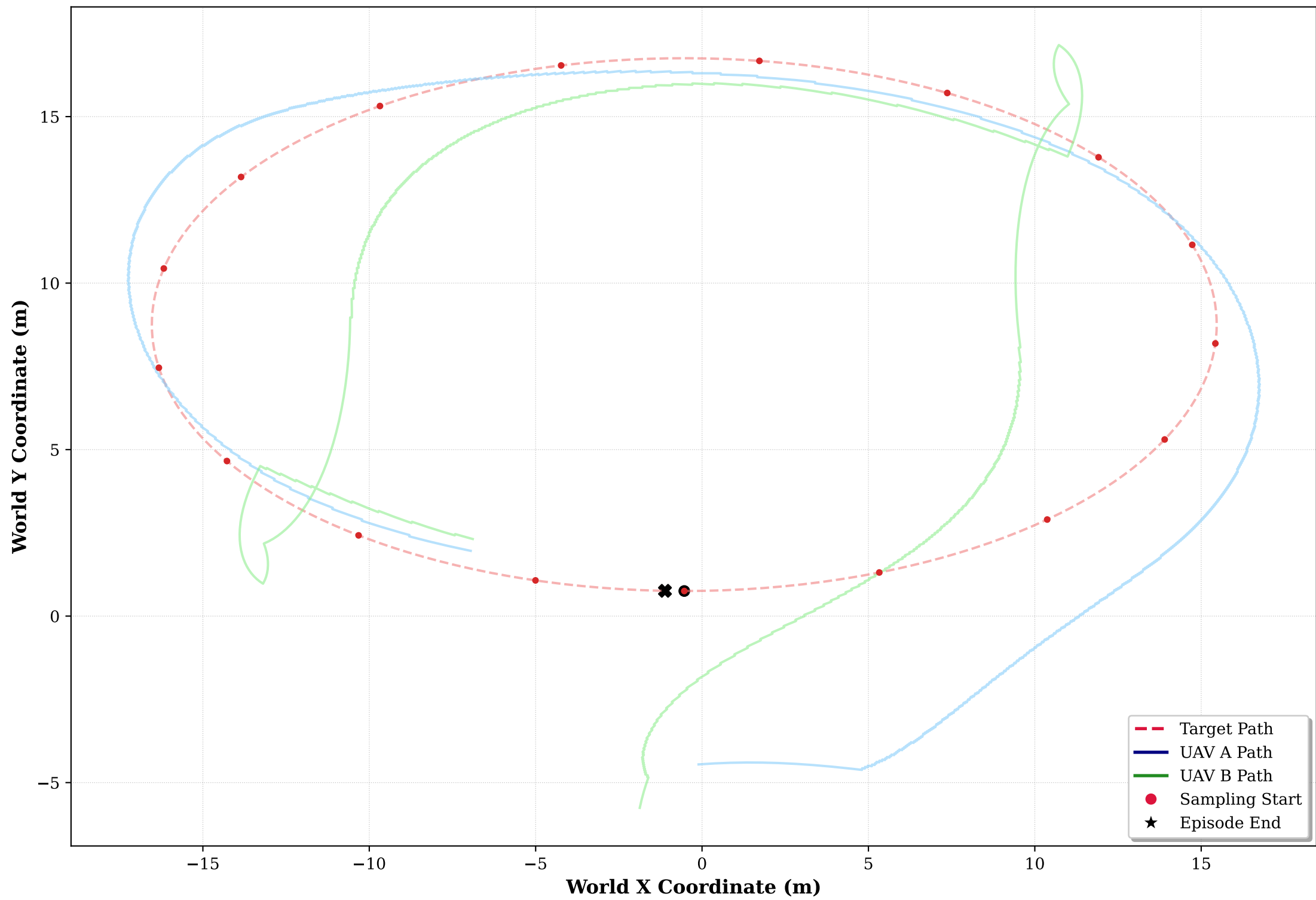
Hierarchical Trajectory Dataset Analysis (Episode 7)
