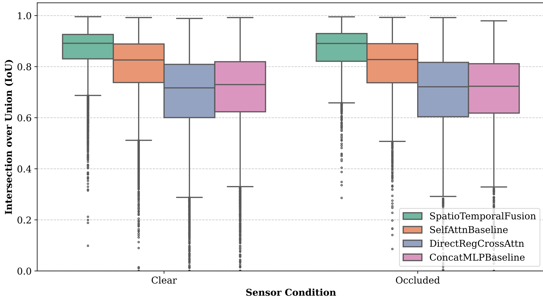
Tracking Accuracy (IoU) Comparison Across Models
