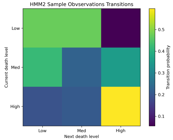
(c) Sampled HMM2 Transition Matrix
