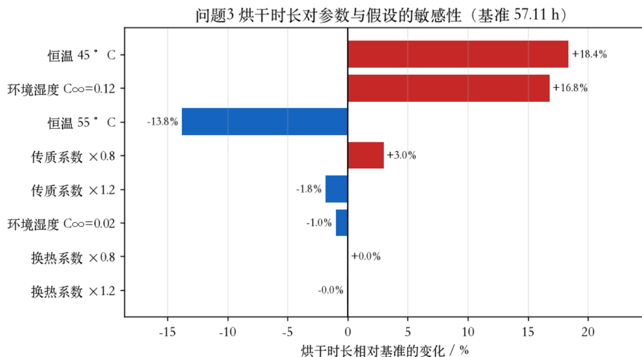
Figure 14: 敏感性
