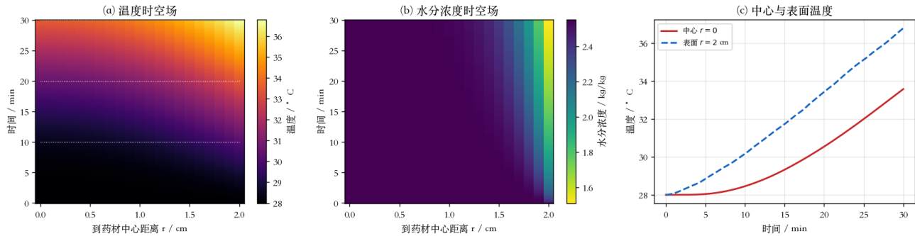
Figure 6: 问题 1 场图
