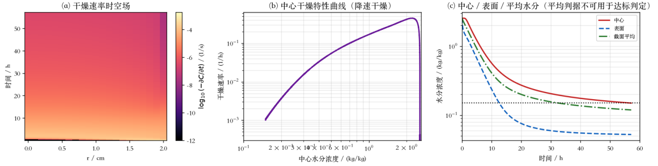
Figure 10: 干燥速率场
