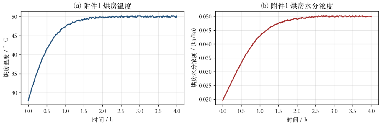
Figure 1: 烘房环境
