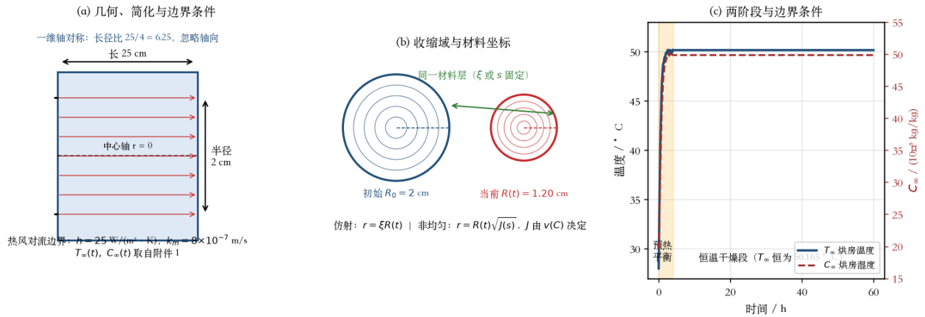
Figure 4: 模型示意
