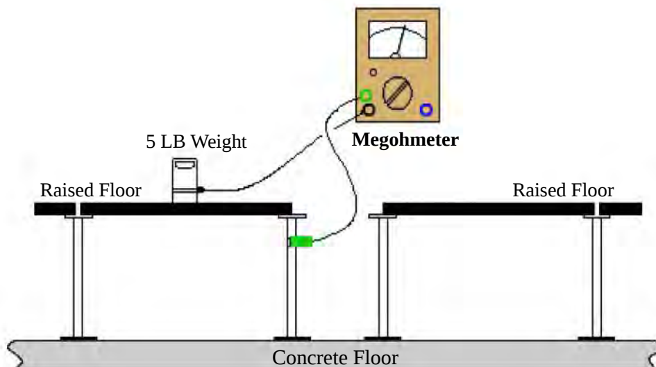
Figure 1. Typical test connection to measure floor conductivity
