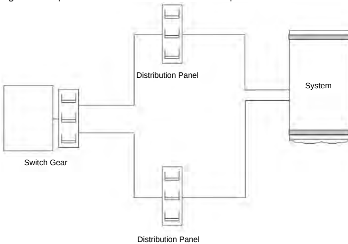
Figure 2. Dual power installation - Redundant distribution panel
