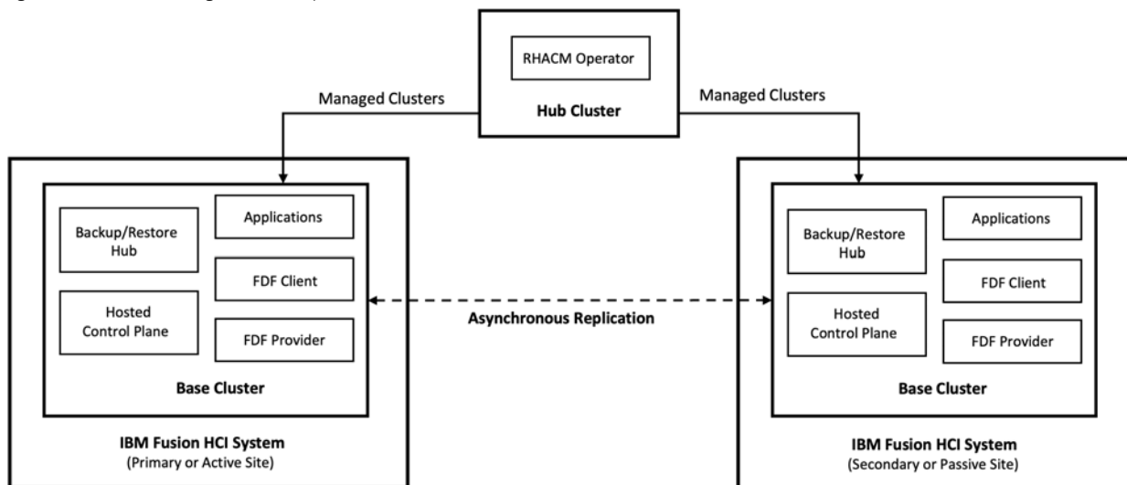
Figure 2. Illustration of a Regional-DR setup for Hosted Control Plane clusters
