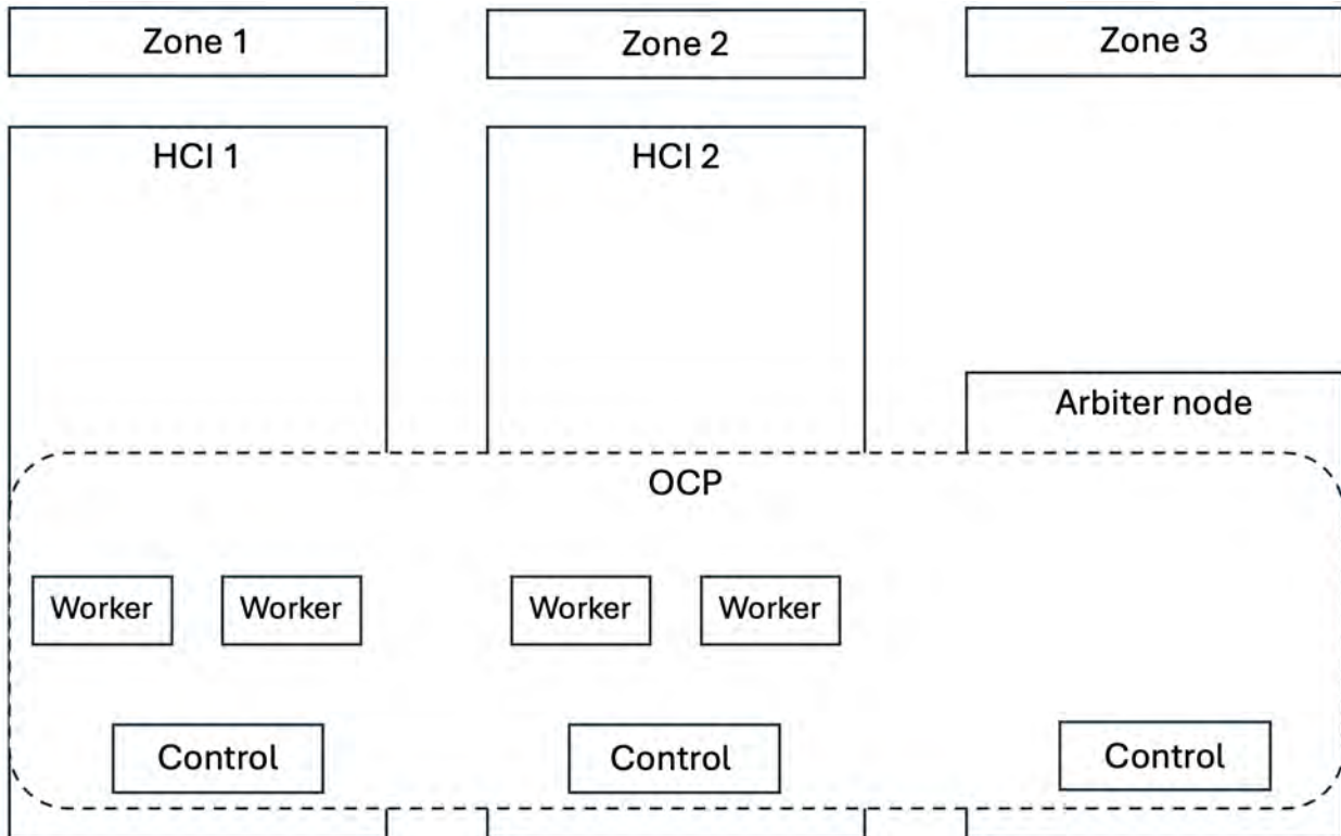
Figure 1. Sample 2AZ and arbiter node configuration
