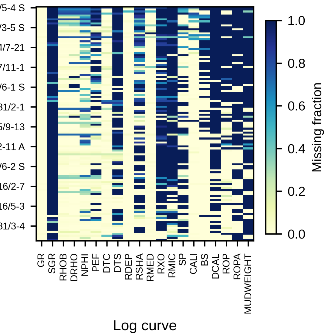
(c) Structured curve-suite missingness
