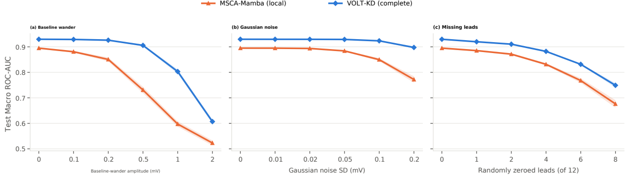
Figure 12: Test macro ROC-AUC under input perturbations for complete VOLT-KD and local MSCA-Mamba. Blue diamonds denote VOLT-KD and orange triangles local MSCA-Mamba; points are five-seed means and shaded bands indicate \pm 1 standard deviation. Panels show (a) low-frequency baseline wander, (b) Gaussian noise, and (c) random lead zeroing. Zero intensity denotes the original test inputs, and model weights are fixed. Complete values appear in Table S6.
