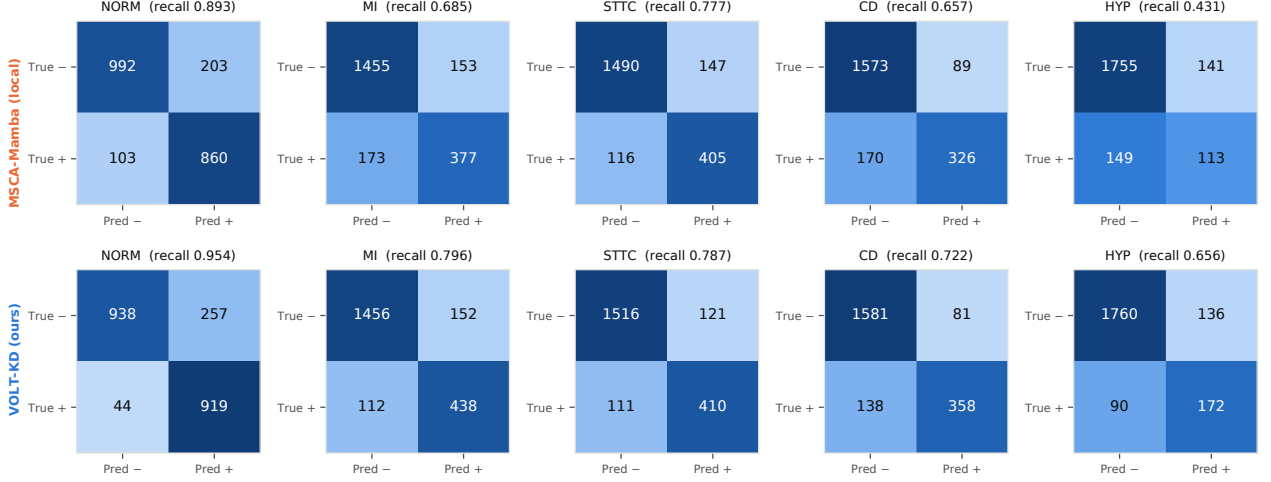
Figure S5: Seed-42 binary confusion matrices for local MSCA-Mamba and VOLT-KD. Each class uses its validation-selected threshold.
