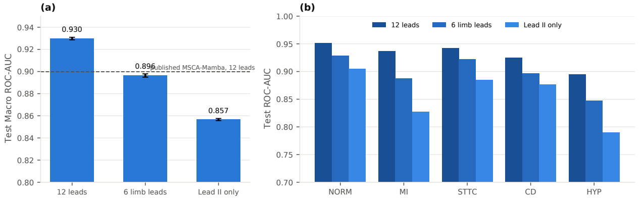
Figure S7: Aggregate and classwise performance of complete twelve-lead VOLT-KD and its six-limb-lead and lead-II student variants. All configurations use twelve-lead ECGFounder soft labels. Aggregate metrics correspond to Table 10.
