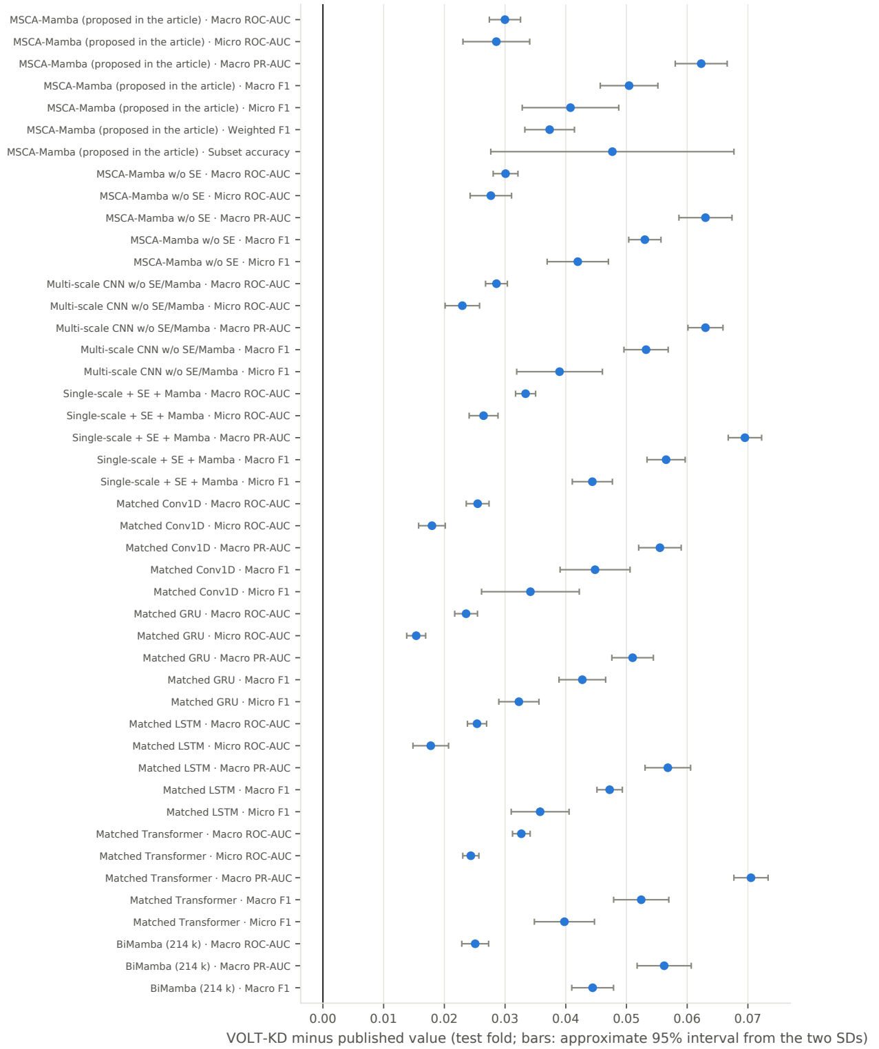
Figure S6: Differences from 45 reported means across nine configurations in the MSCA-Mamba paper[2]. Matched metrics are compared; points are VOLT-KD minus published values, with approximate intervals constructed from reported standard deviations.
