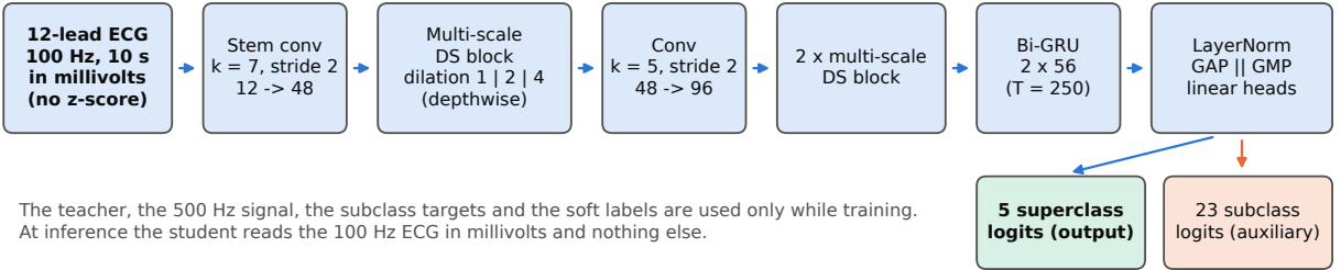
Figure 1: Amplitude-preserving training and inference. Higher-rate recordings, teacher soft labels, and diagnostic subclasses are used only during training. Inference maps a 100 Hz ECG to five diagnostic superclasses. Complete VOLT-KD uses superclass, subclass, and teacher supervision.
