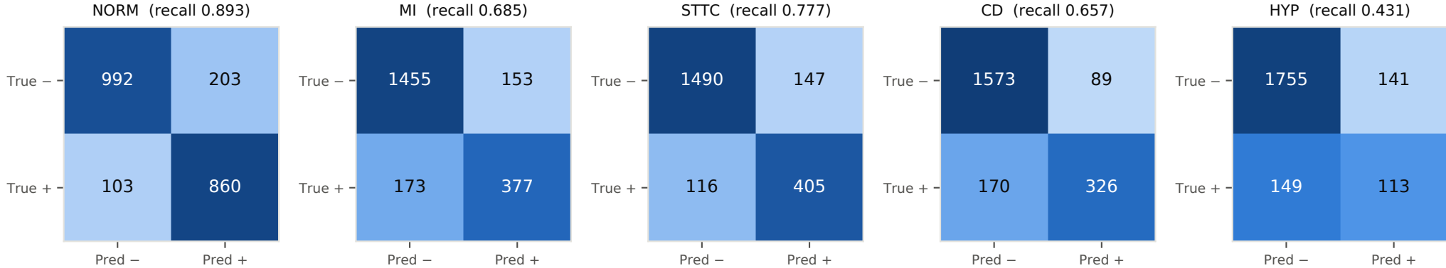
MSCA-Mamba (local)
