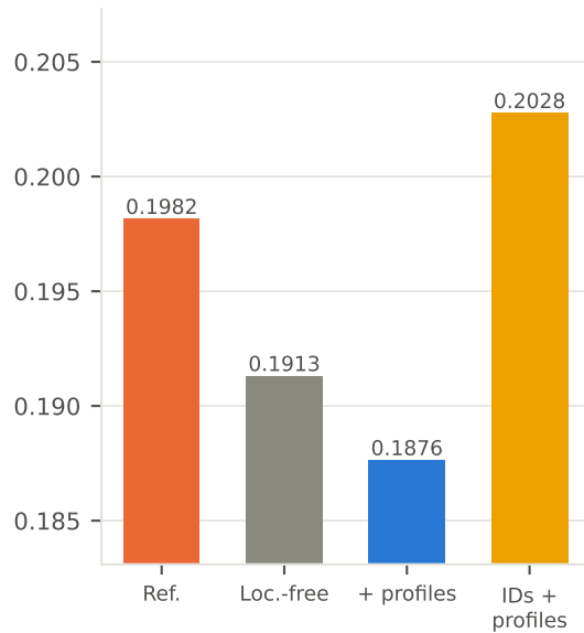
Log loss ↓
