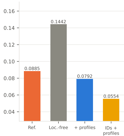
|Calibration slope - 1| ↓
