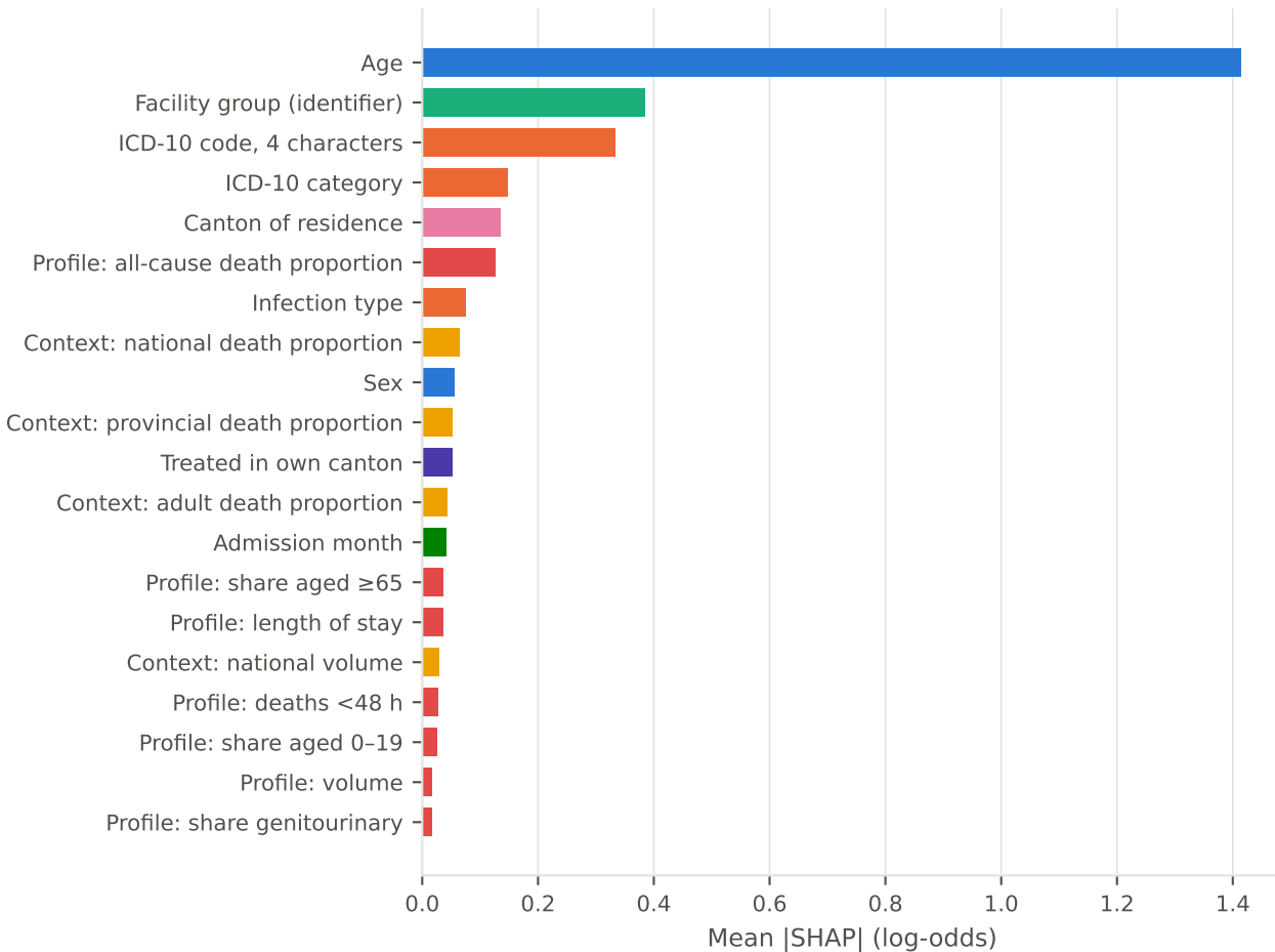
Top 20 features of the LightGBM member
