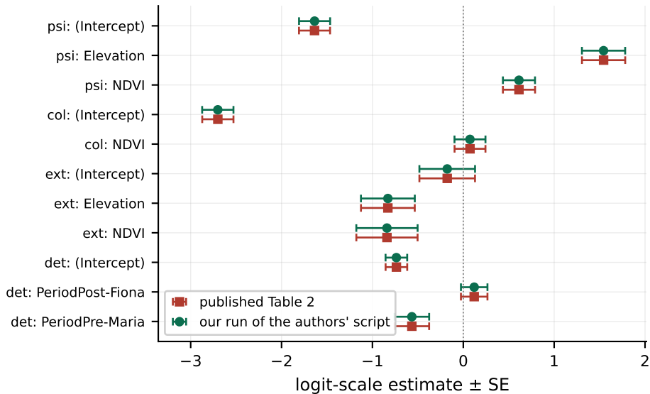
Dynamic occupancy model: 11/11 estimates and 11/11 SEs reproduce exactly
