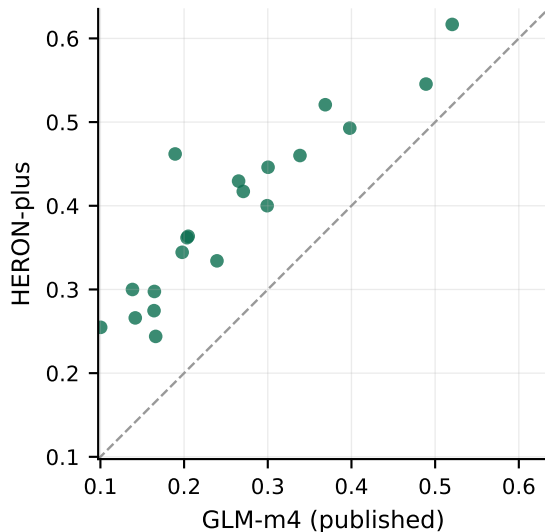
AP: HERON-plus wins 20/20 folds
