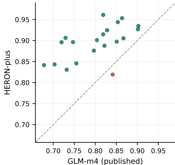
AUC: HERON-plus wins 19/20 folds
