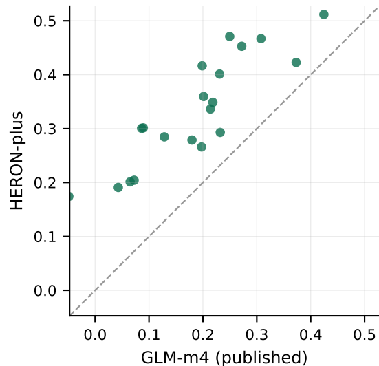
pseudoR2: HERON-plus wins 20/20 folds
