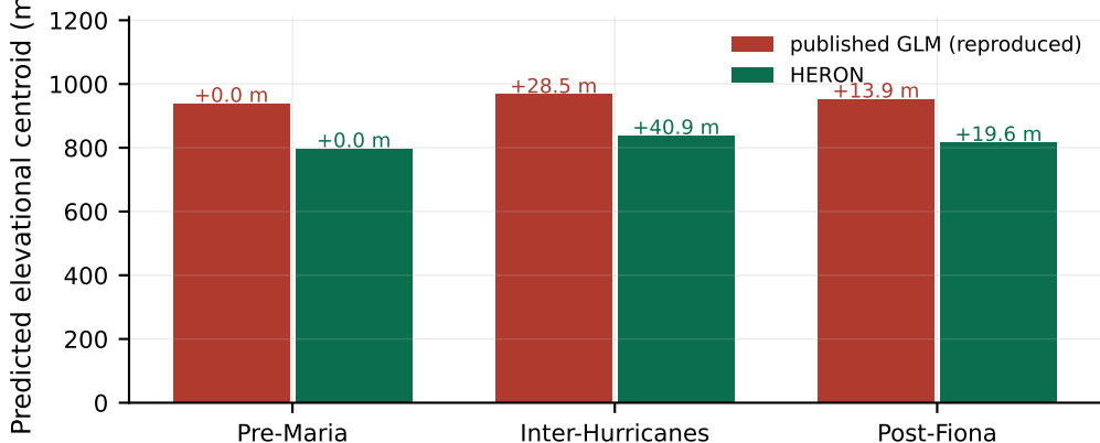
Elevational centroid by period (published Figure 4 statistic) labels show the shift relative to each model's own Pre-María baseline
