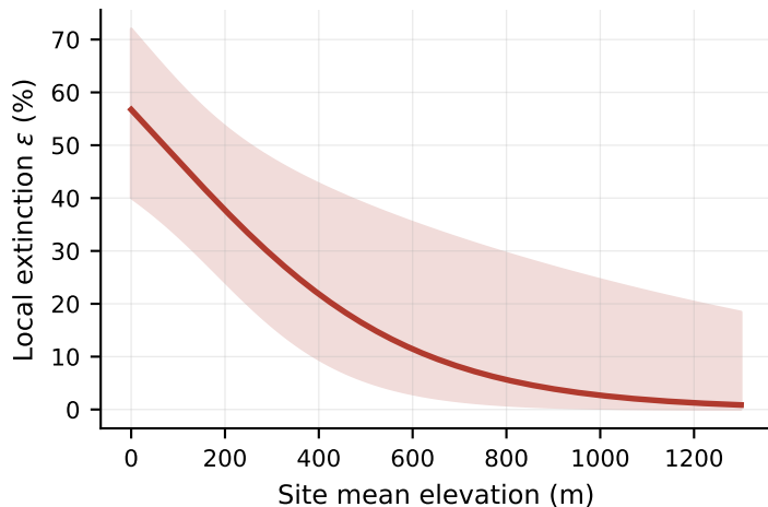
(a) Published dynamic occupancy model (reproduces Figure 5)
