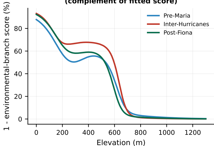
(b) HERON's environmental branch (complement of fitted score)
