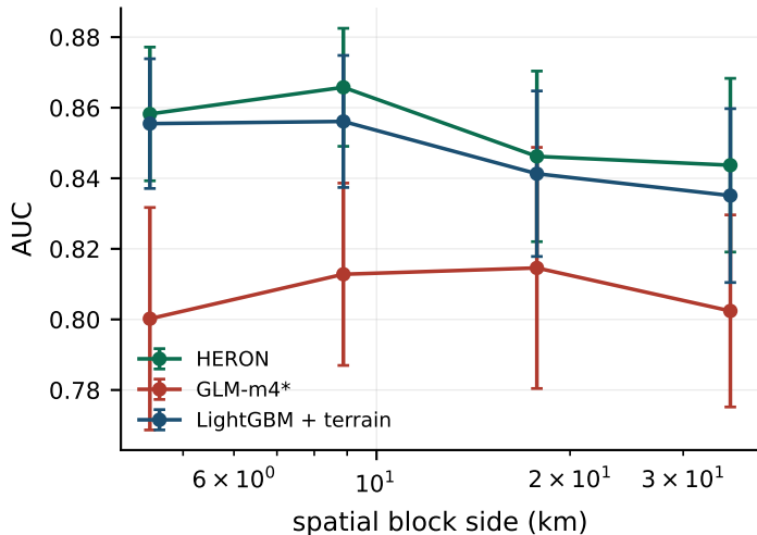
AUC vs spatial-block size
