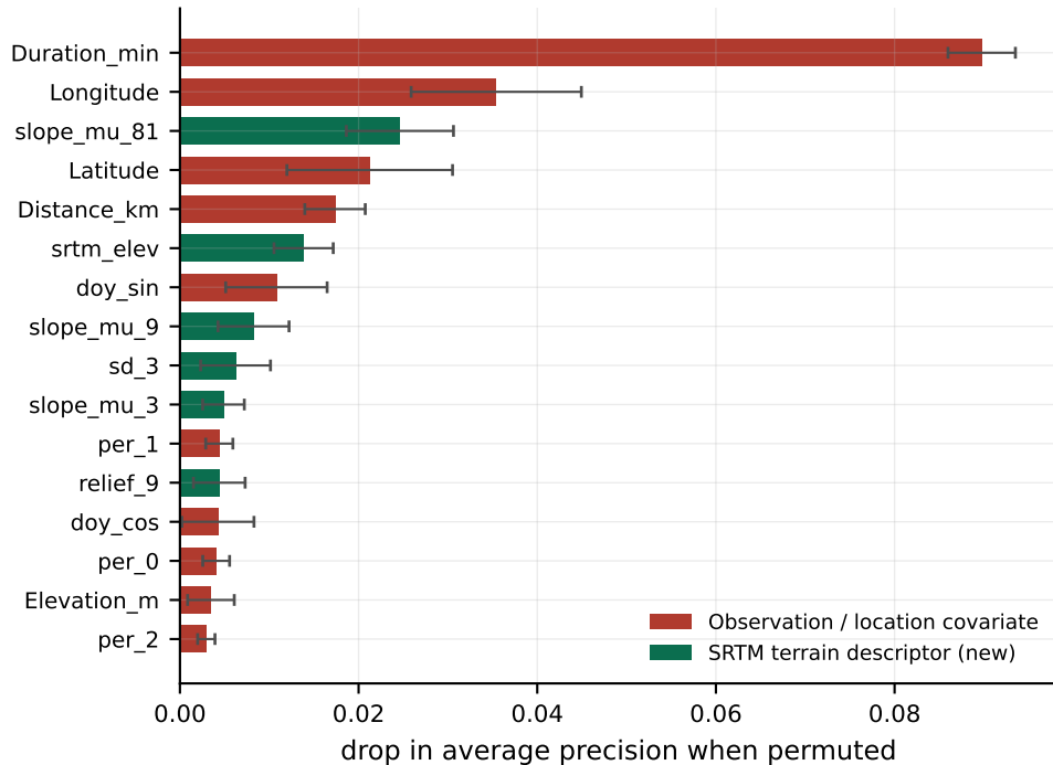
(b) LightGBM + terrain member (where terrain enters the stack)
