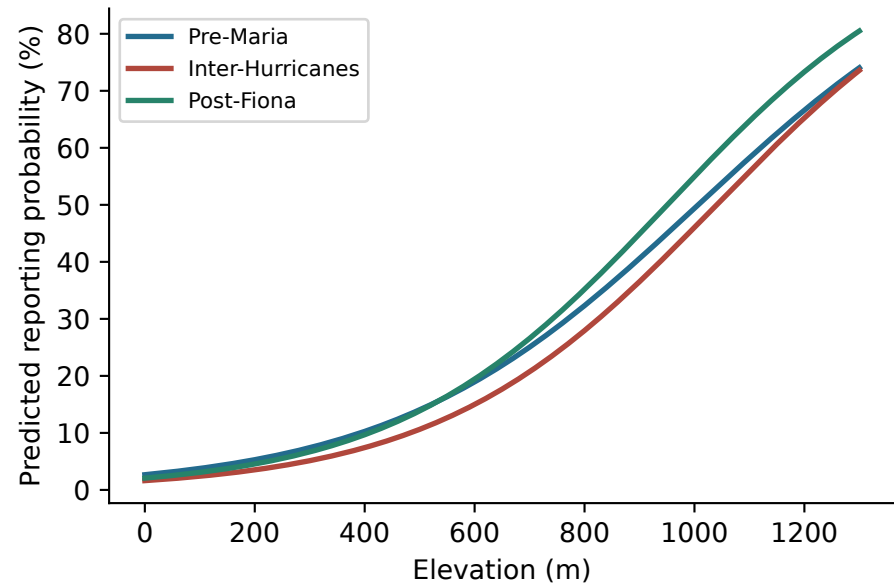
(a) Reproduced conditional GLM curves
