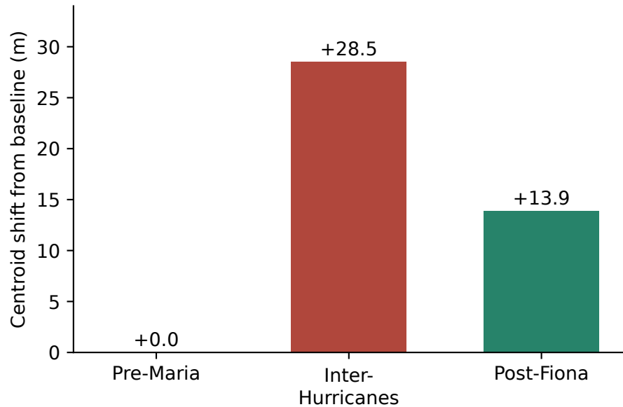
(b) Probability-weighted centroid shifts
