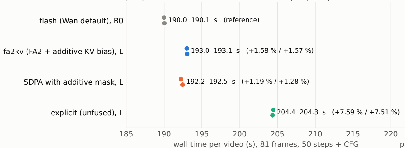
(a) Time per video by attention path
