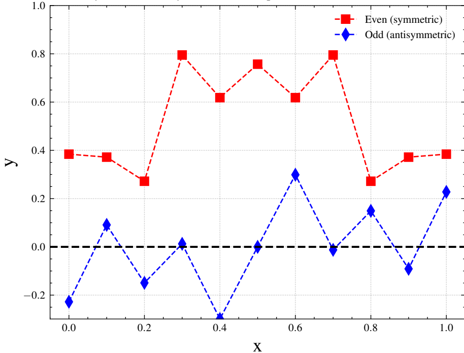
Symmetric-Antisymmetric Decomposition of a Discrete Function
