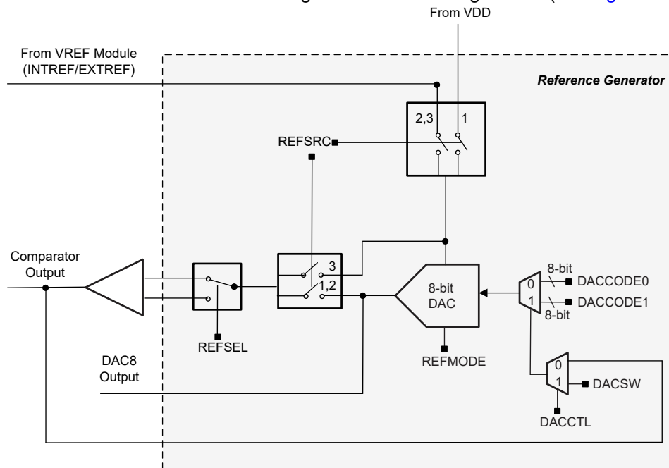
Figure 18-3. Reference Voltage Generator Block Diagram
