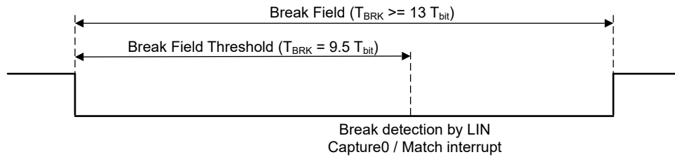
Figure 23-6. LIN Break Field Detection
