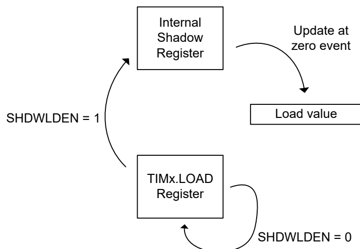
Figure 27-24. Load value updates for TIMx instances when EN=1
