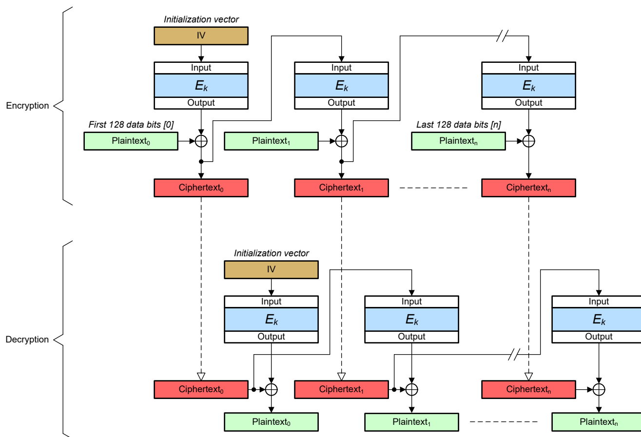
Figure 12-5. CFB Cipher
