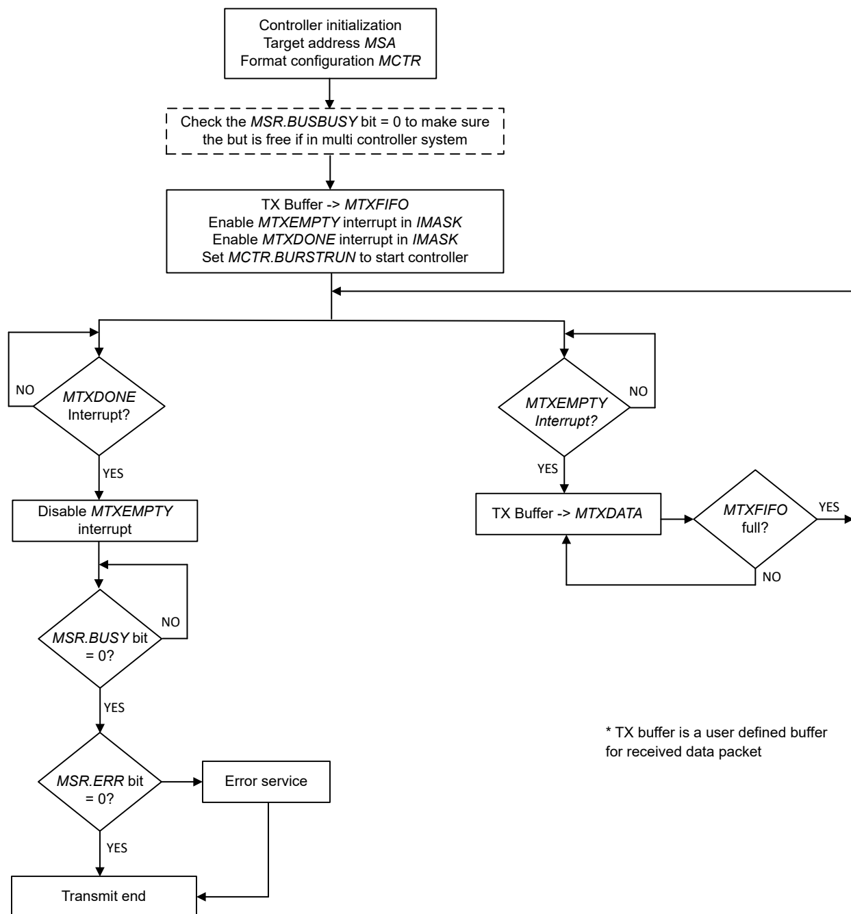
Figure 24-12. Controller Transmitter Mode
