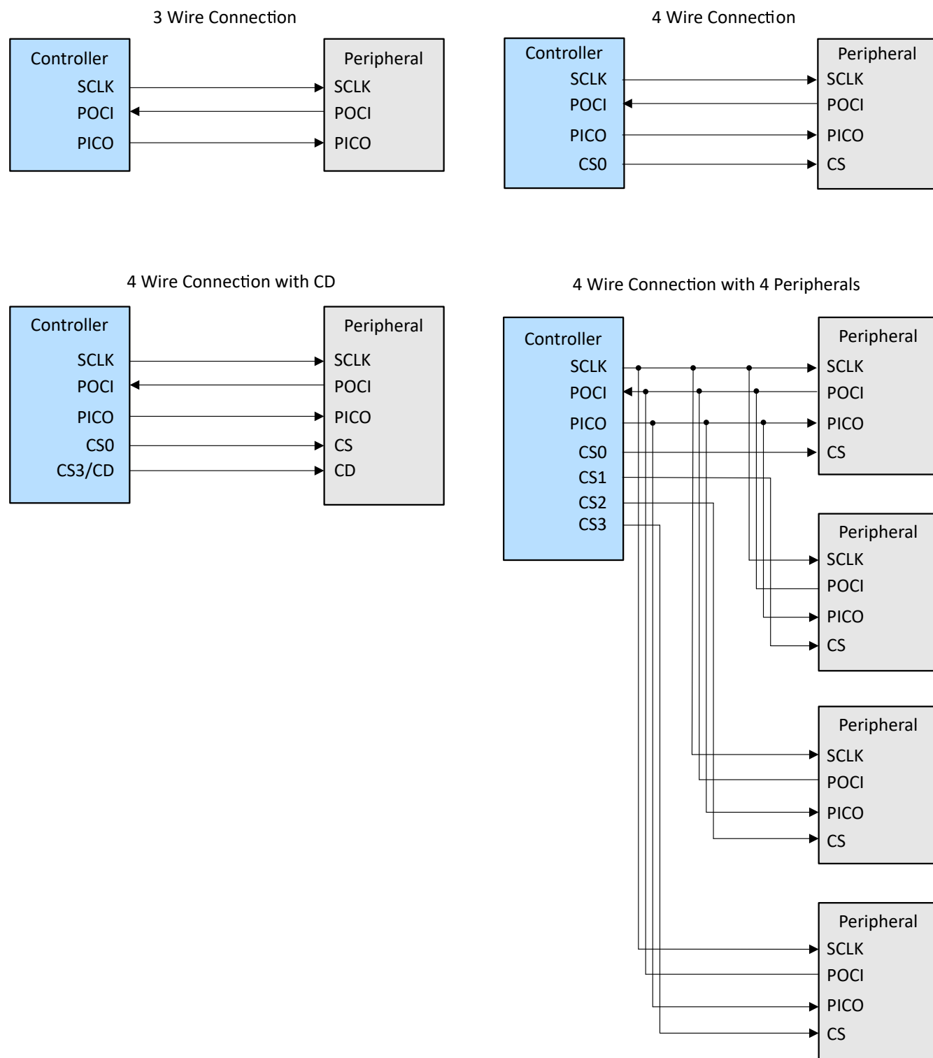
Figure 25-2. External Connections for Different SPI Configurations
