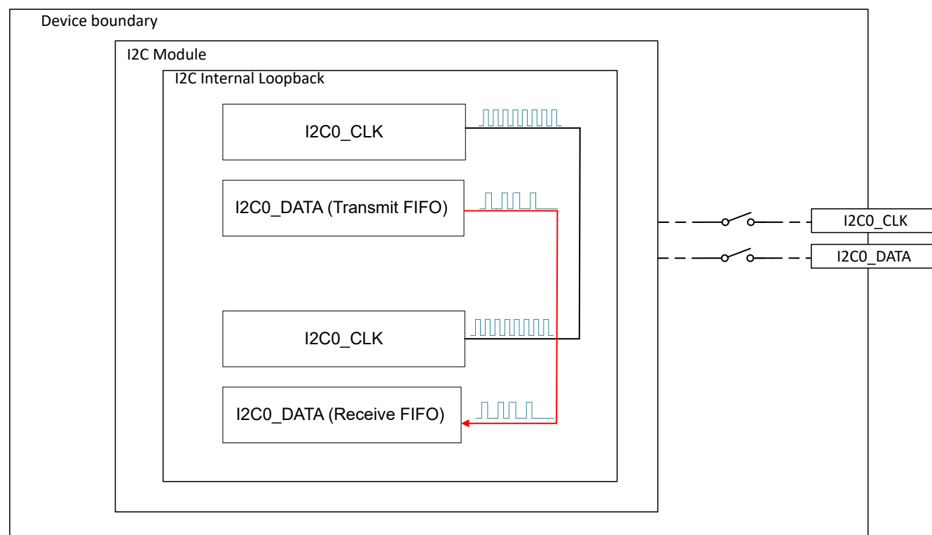
Figure 24-10. I2C Internal Loopback mode
