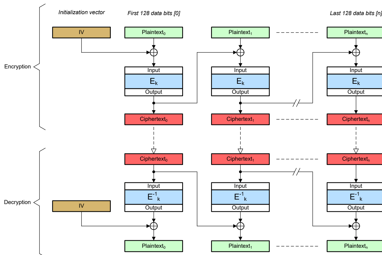
Figure 12-3. CBC Cipher
