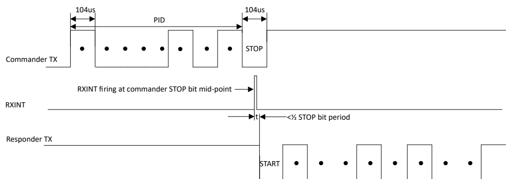
Figure 23-8. LIN Responder Transmission Delay
