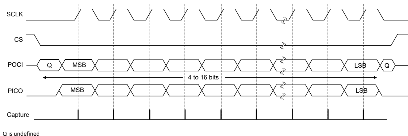
Figure 25-4. Motorola SPI Format With SPO = 0 and SPH = 0
