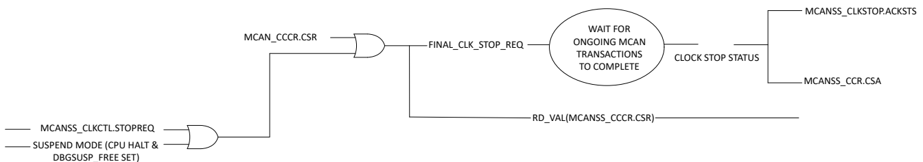
Figure 26-8. Clock Stop Request
