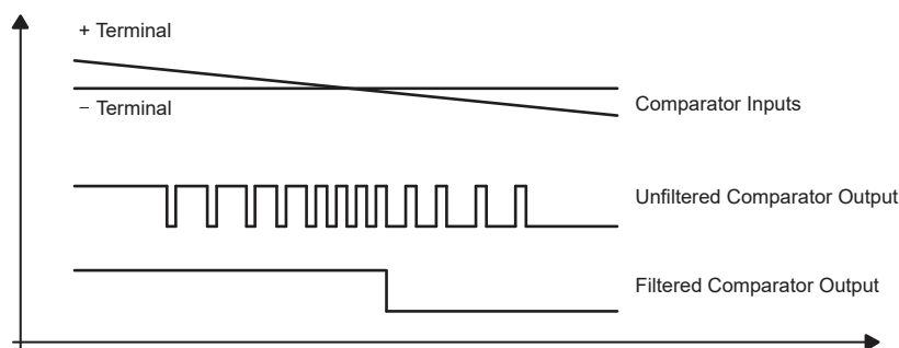
Figure 18-2. Analog Filter Response at the Output of the Comparator
