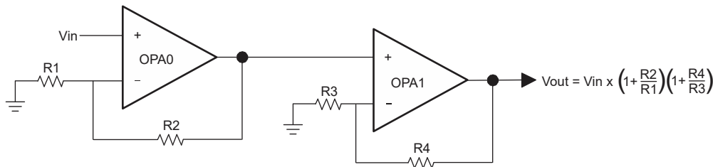
Figure 20-9. Two OPA Non-inverting to Non-inverting Cascade Amplifier Block Diagram and Equation
