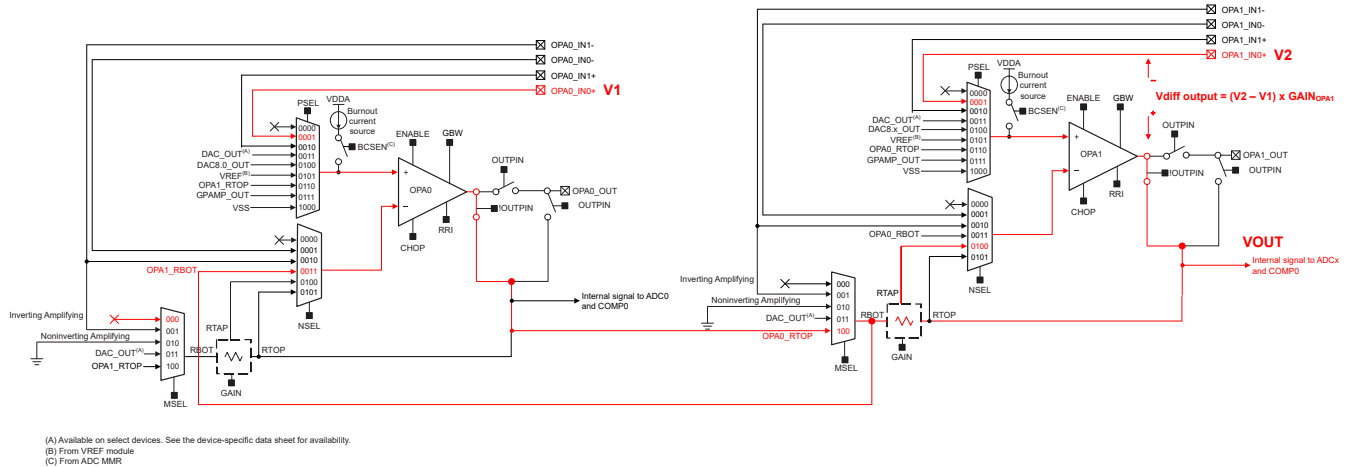
Figure 20-8. Two OPAs in Difference Amplifier Configuration
