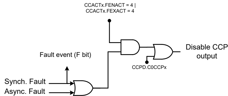
Figure 27-36. Fault Output Generation Connections
