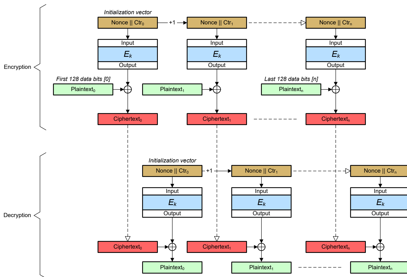
Figure 12-6. CTR Cipher
