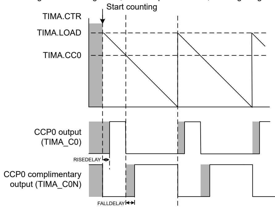
Figure 27-32. Deadband Insertion (Mode 0) for PWM in Down-Counting Mode
