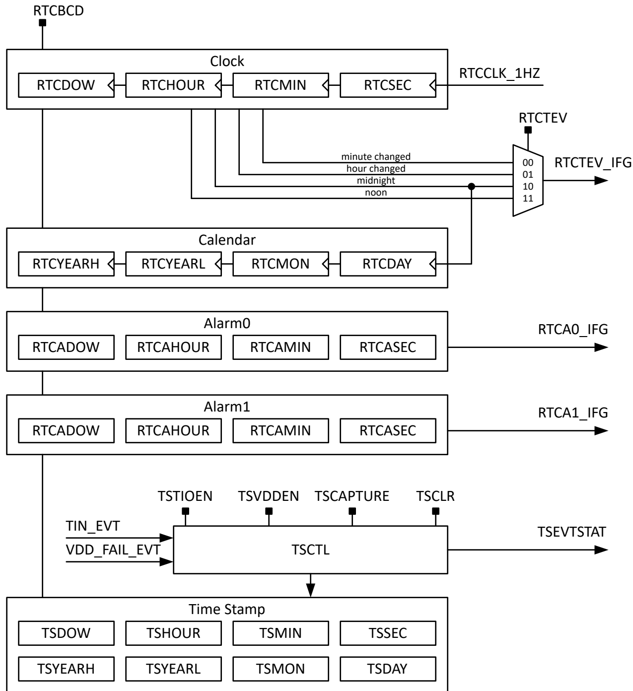
Figure 29-4. RTC Block Diagram and Timestamping
