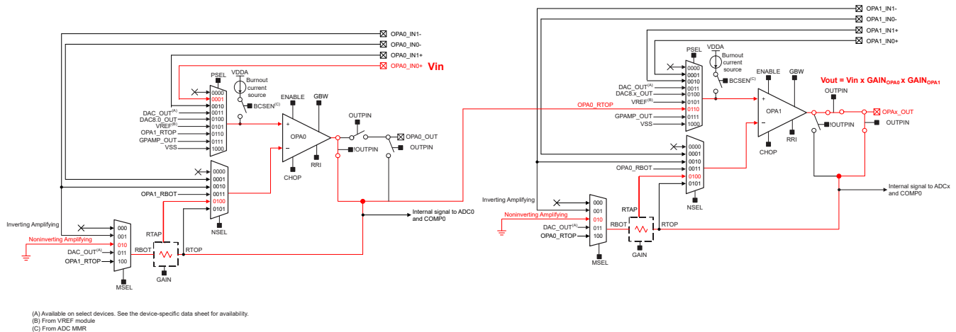
Figure 20-10. Two OPAs in Non-inverting to Non-inverting Cascade Amplifier Configuration
