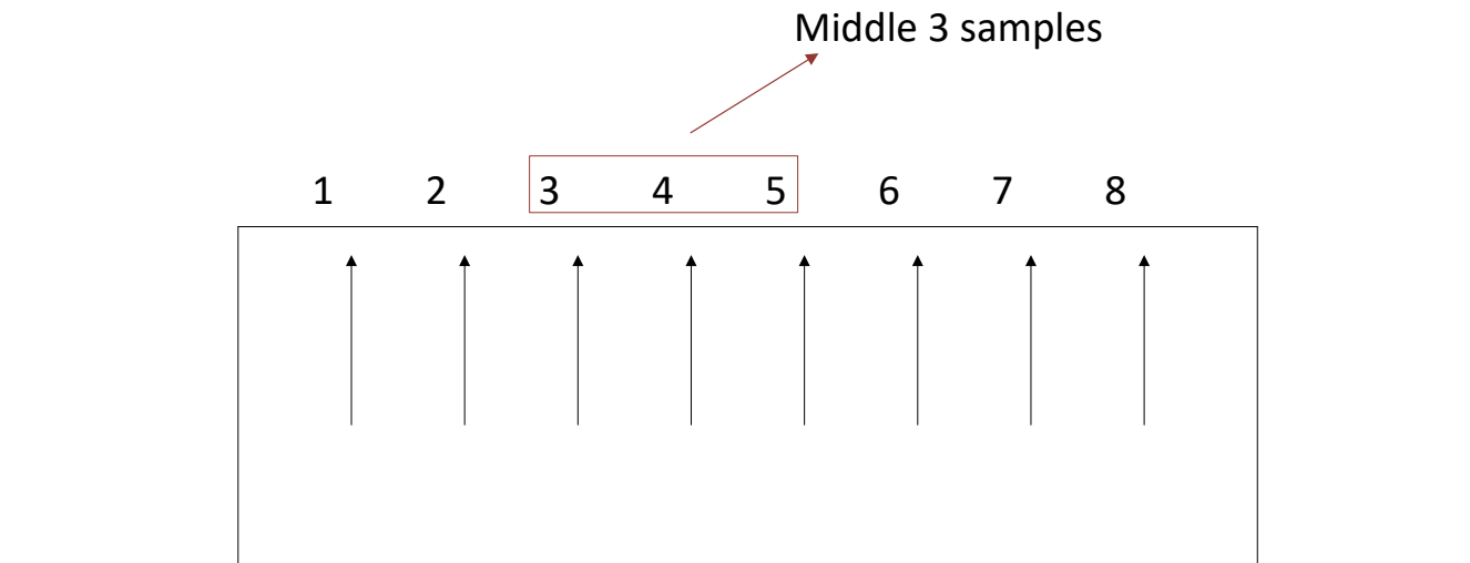
Figure 23-4. Majority voting for 8 oversampling
