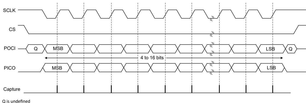
Figure 25-7. Motorola SPI Frame Format With SPO = 1 and SPH = 1
