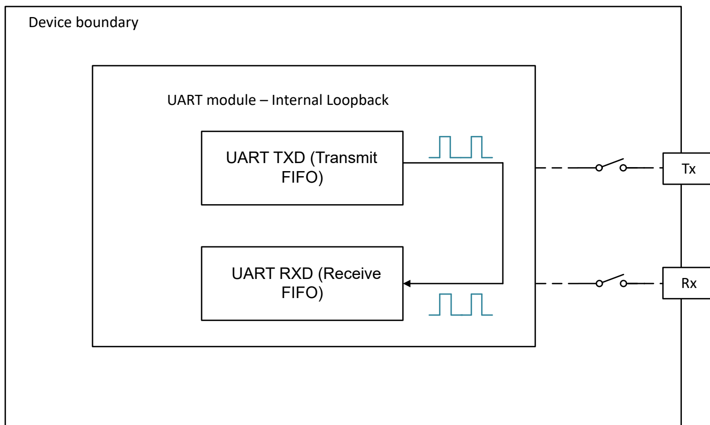
Figure 23-15. UART Loopback mode
