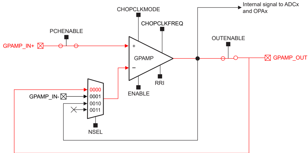
Figure 21-4. GPAMP in Unity Gain Configuration
