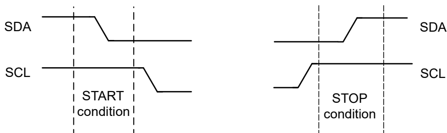
Figure 24-5. START and STOP Conditions
