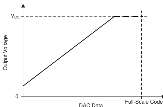
Figure 19-7. Positive Offset
