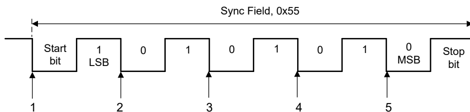
Figure 23-7. LIN SYNC Field Detection
