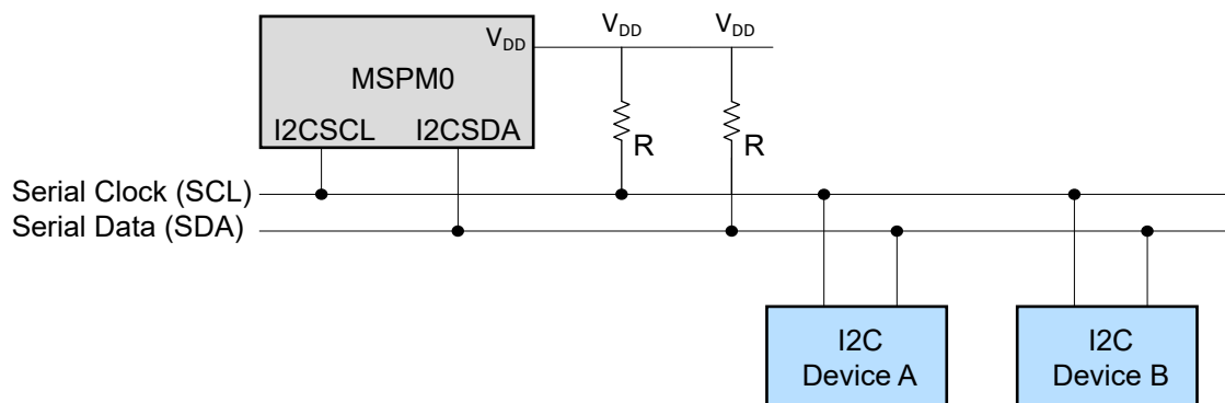
Figure 24-2. Bus Connection Diagram
