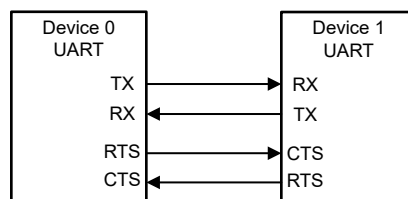
Figure 23-9. Flow Control
