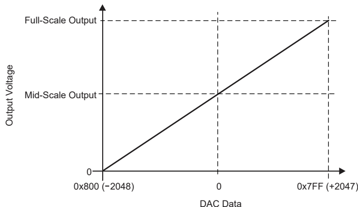
Figure 19-3. Output Voltage vs DAC Data, 12-Bit Twos-Complement Mode
