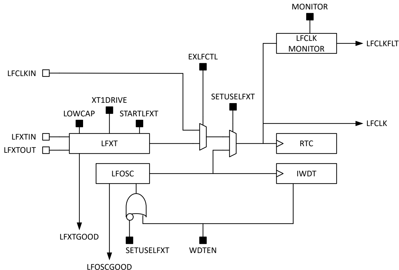
Figure 28-1. LFSS Low-Frequency Clock System
