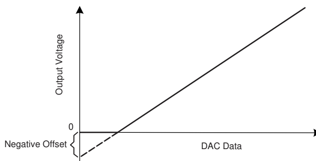
Figure 19-6. Negative Offset
