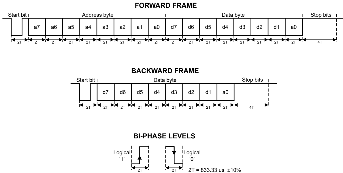
Figure 23-13. DALI Protocol
