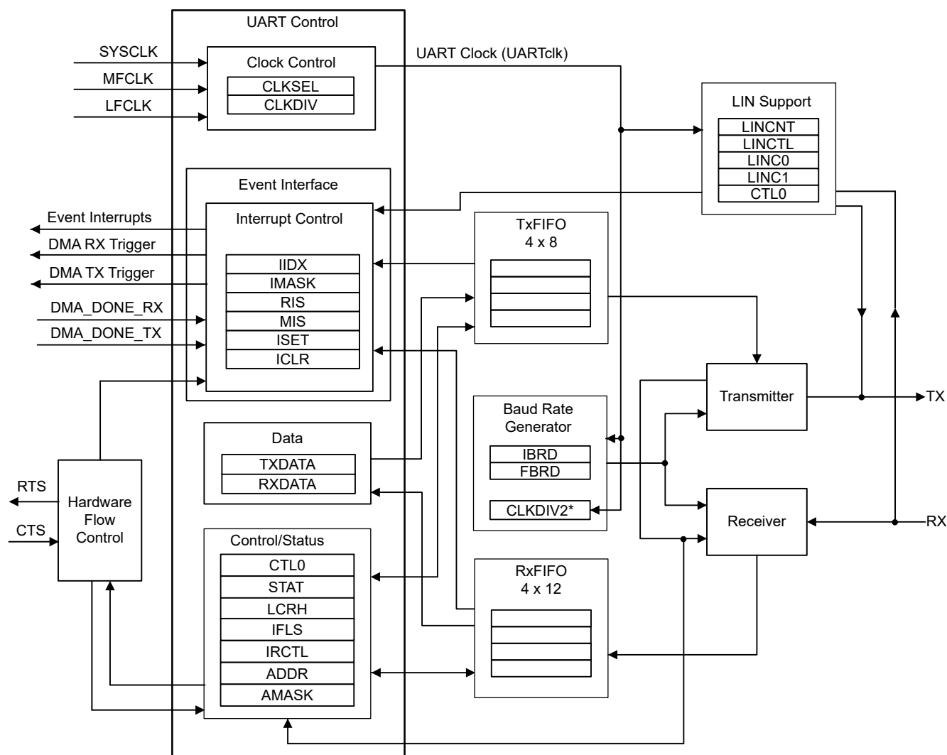
Figure 23-1. UART Functional Block Diagram
