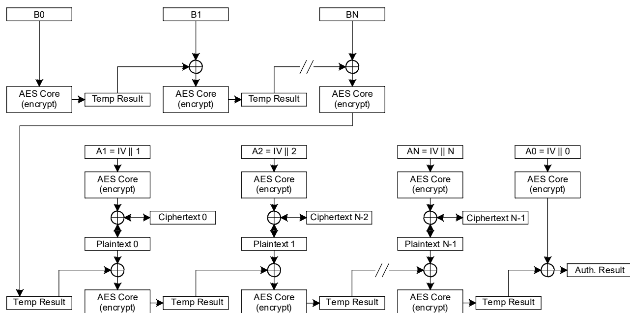
Figure 12-9. CCM Protocol Operation
