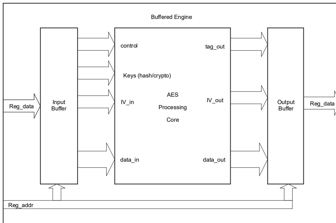
Figure 12-1. AESADV Block Diagram
