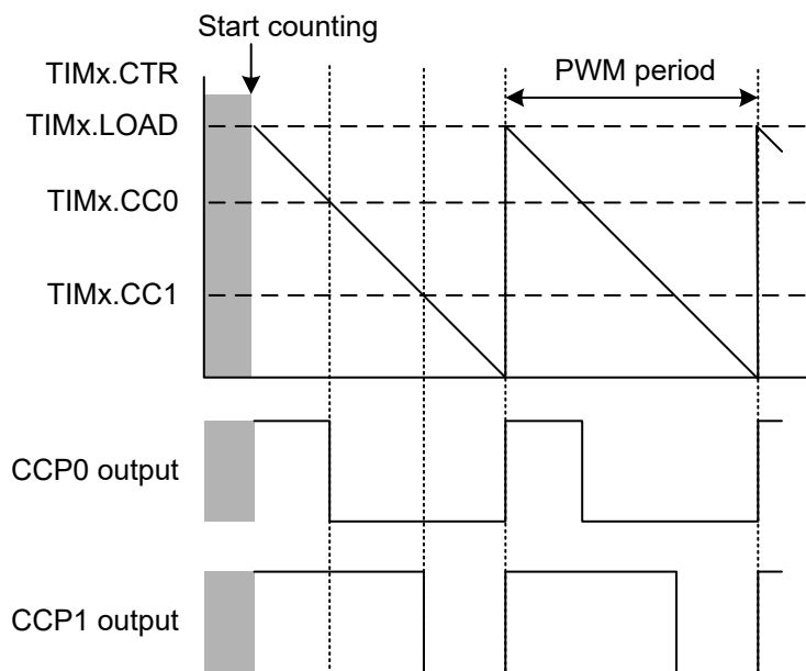
Figure 27-28. Edge-Aligned PWM Signals in Down-Counting Mode
