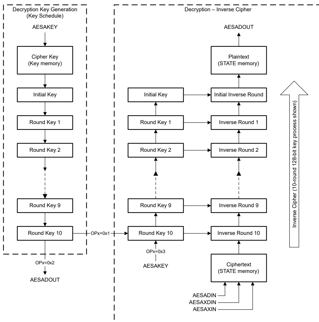
Figure 11-4. AES Decryption (OPx = 0x1, 128-bit Key)
