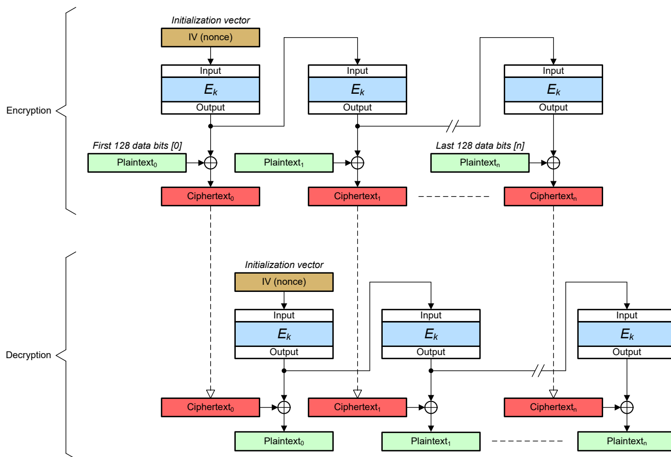
Figure 11-7. OFB Cipher
