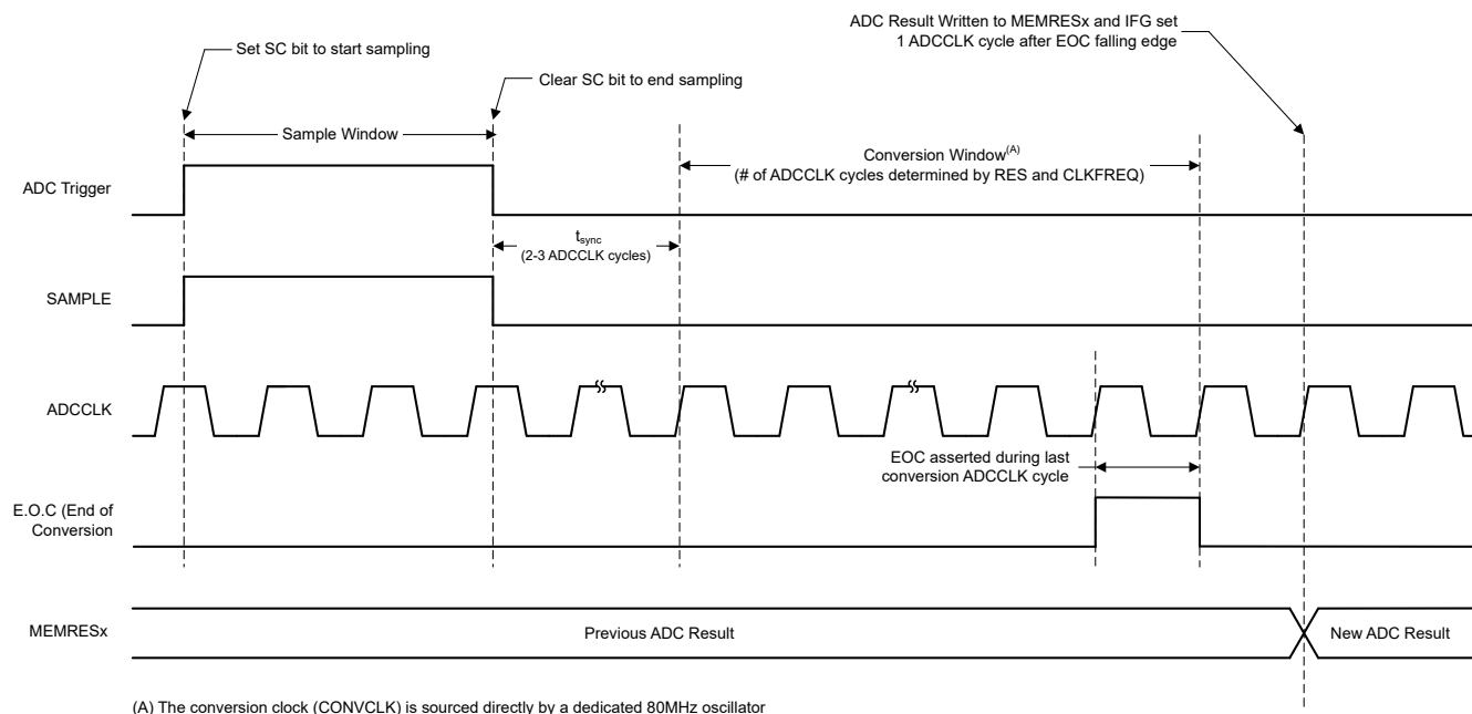
Figure 17-3. MANUAL Sampling Mode ADC Sample and Conversion Timing Diagram
