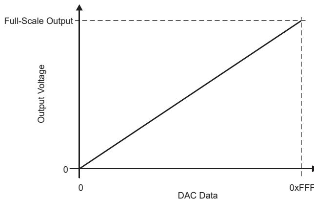
Figure 19-2. Output Voltage vs DAC Data, 12-Bit Straight-Binary Mode
