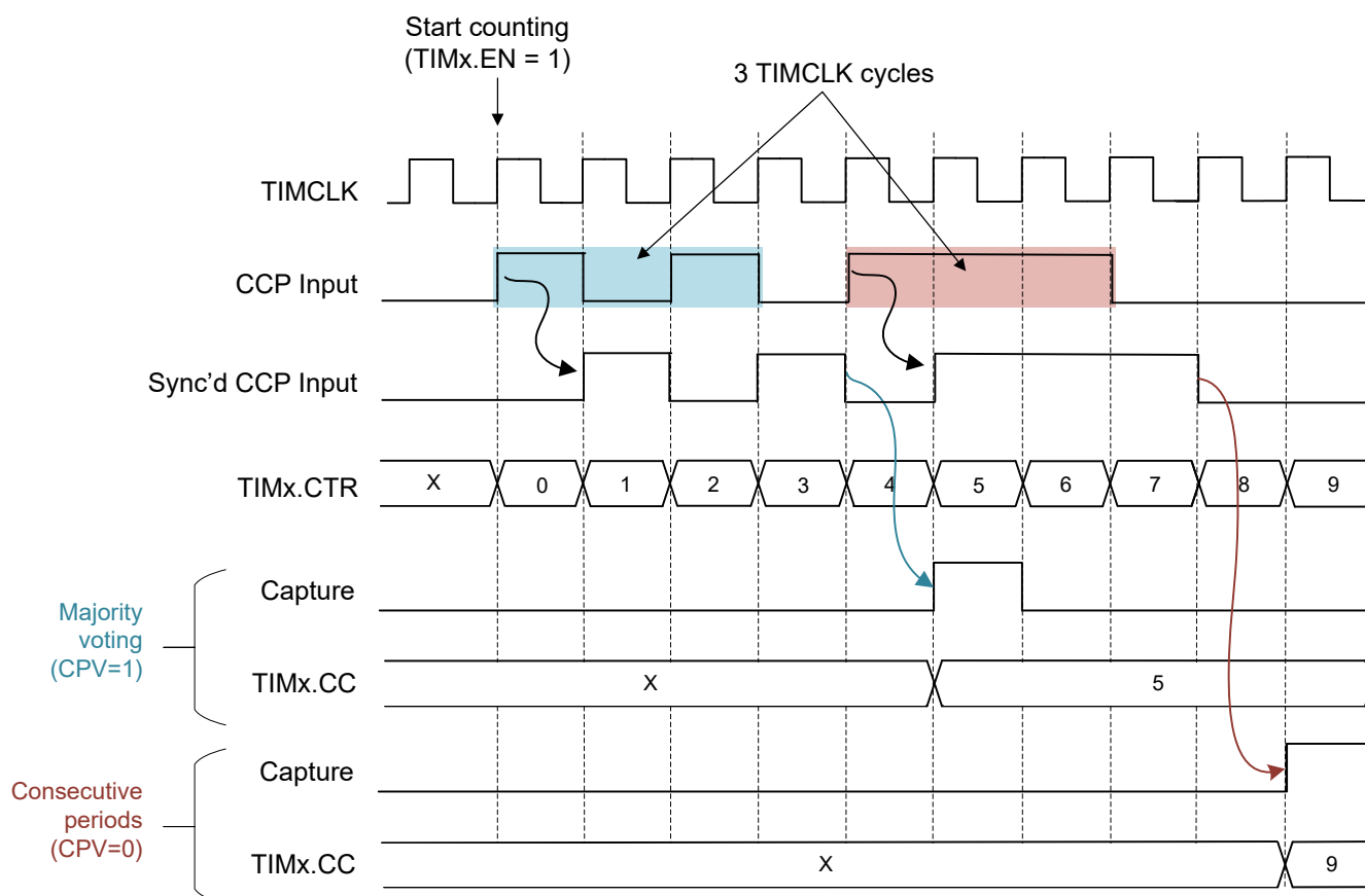
Figure 27-13. Consecutive Period and Majority Voting for Input Glitch Filtering using FP = 0 (3 TIMCLK cycles)
