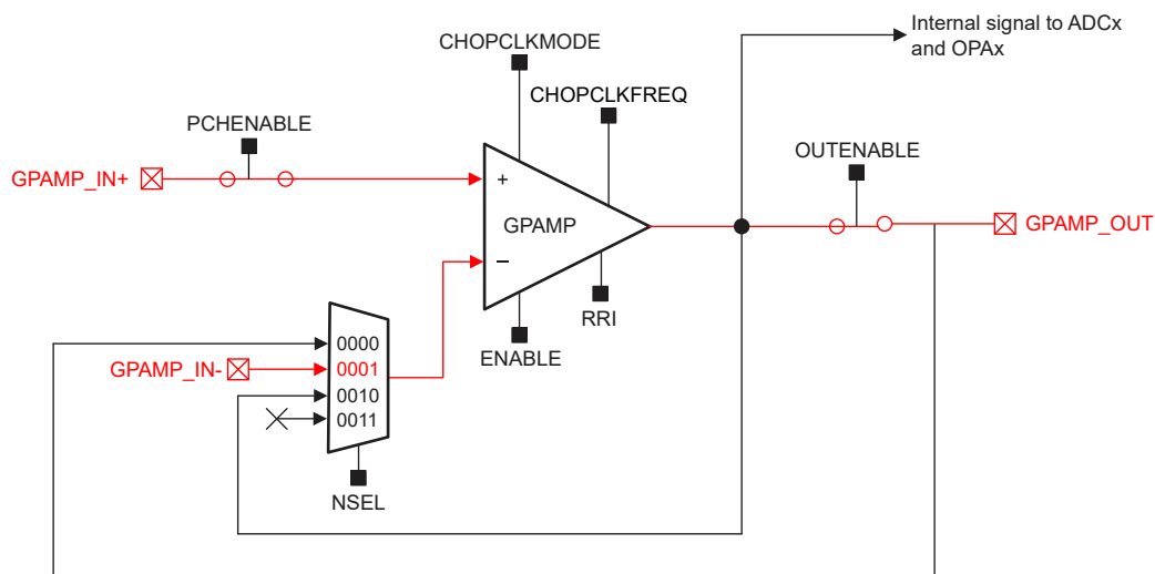
Figure 21-2. GPAMP in General Purpose (GP) Mode
