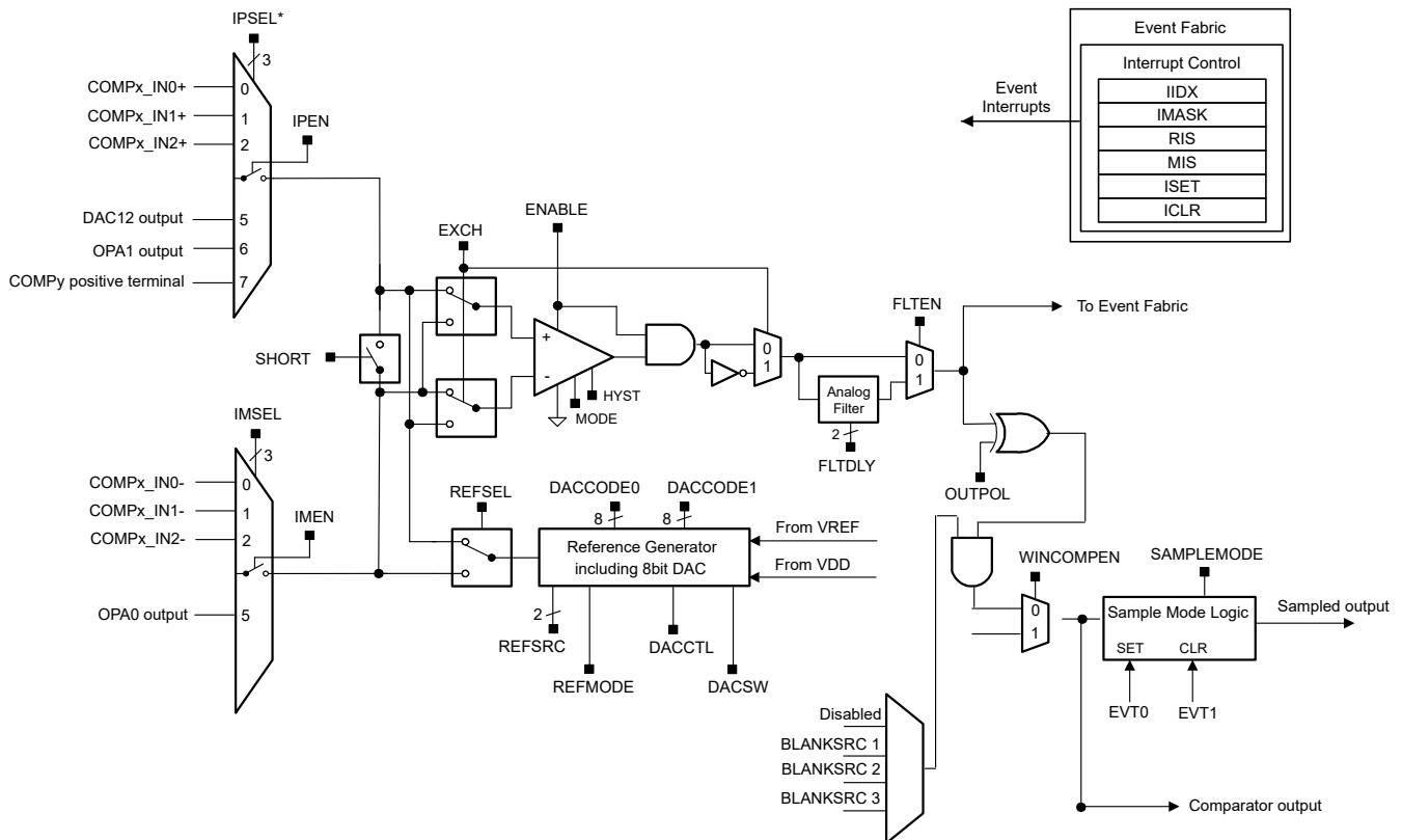
Figure 18-1. Comparator Block Diagram
