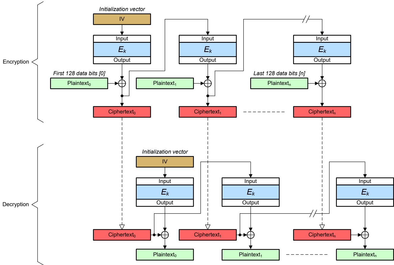
Figure 11-8. CFB Cipher
