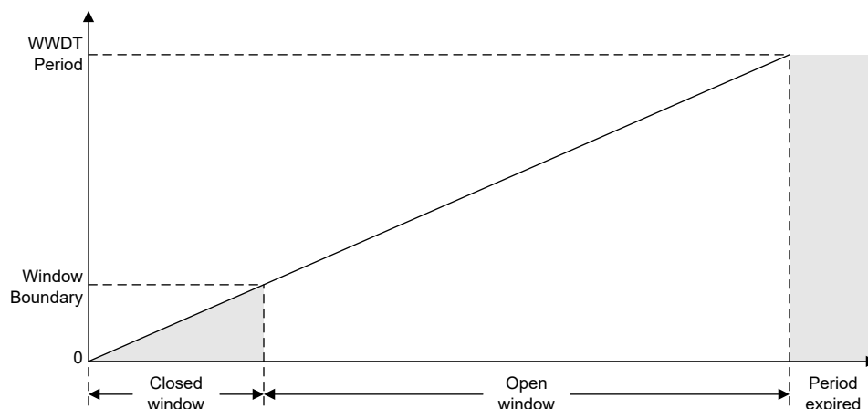
Figure 31-1. WWDT Functionality
