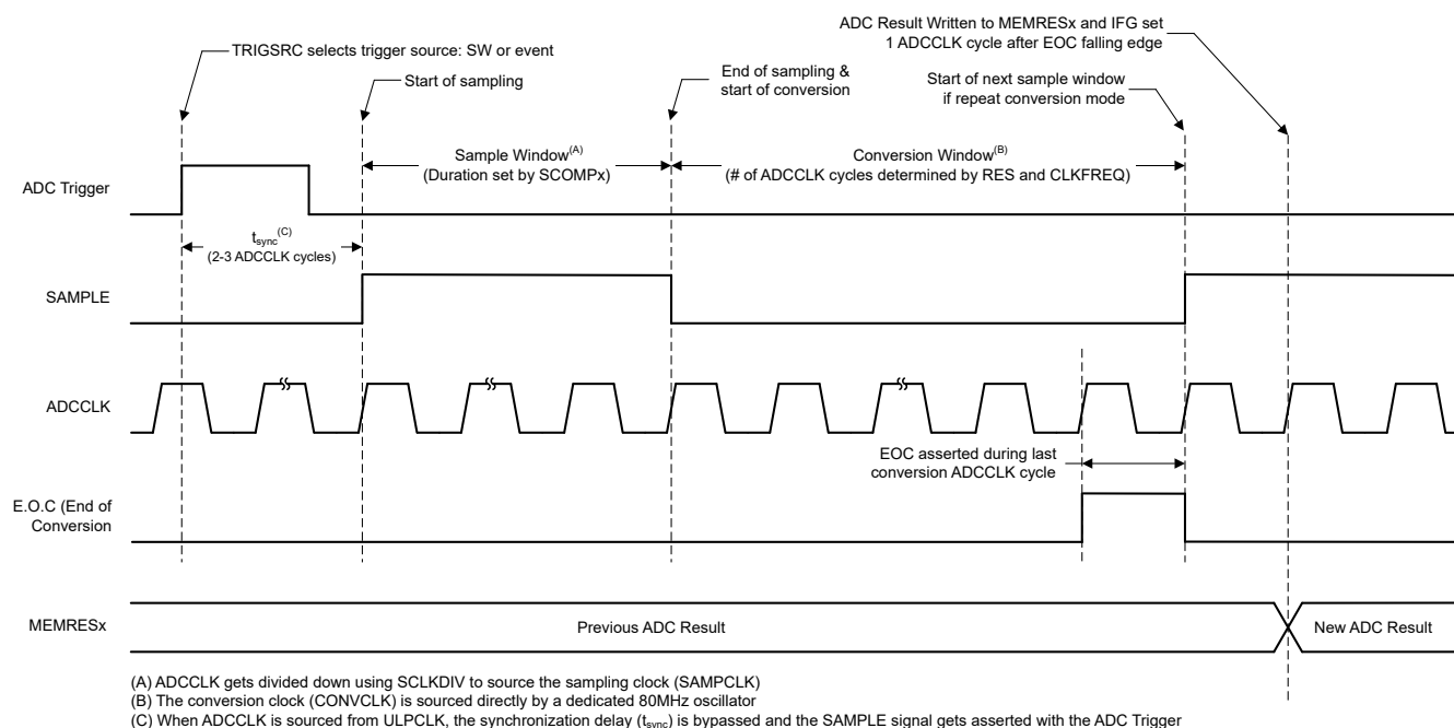
Figure 17-2. AUTO Sampling Mode ADC Sample and Conversion Timing Diagram
