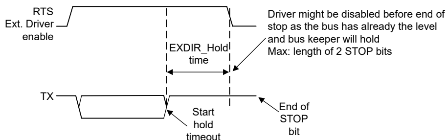
Figure 23-12. RS485 External Control
