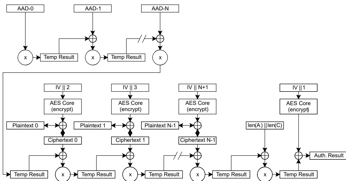
Figure 12-7. GCM Protocol Operation
