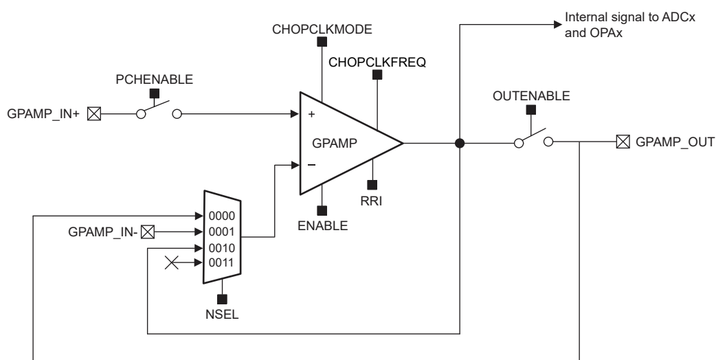
Figure 21-1. GPAMP Block Diagram
