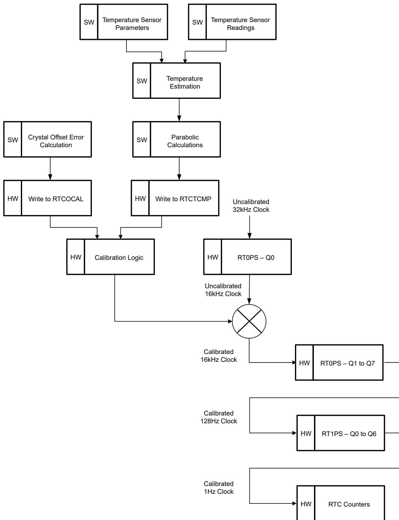
Figure 29-2. RTC Calibration
