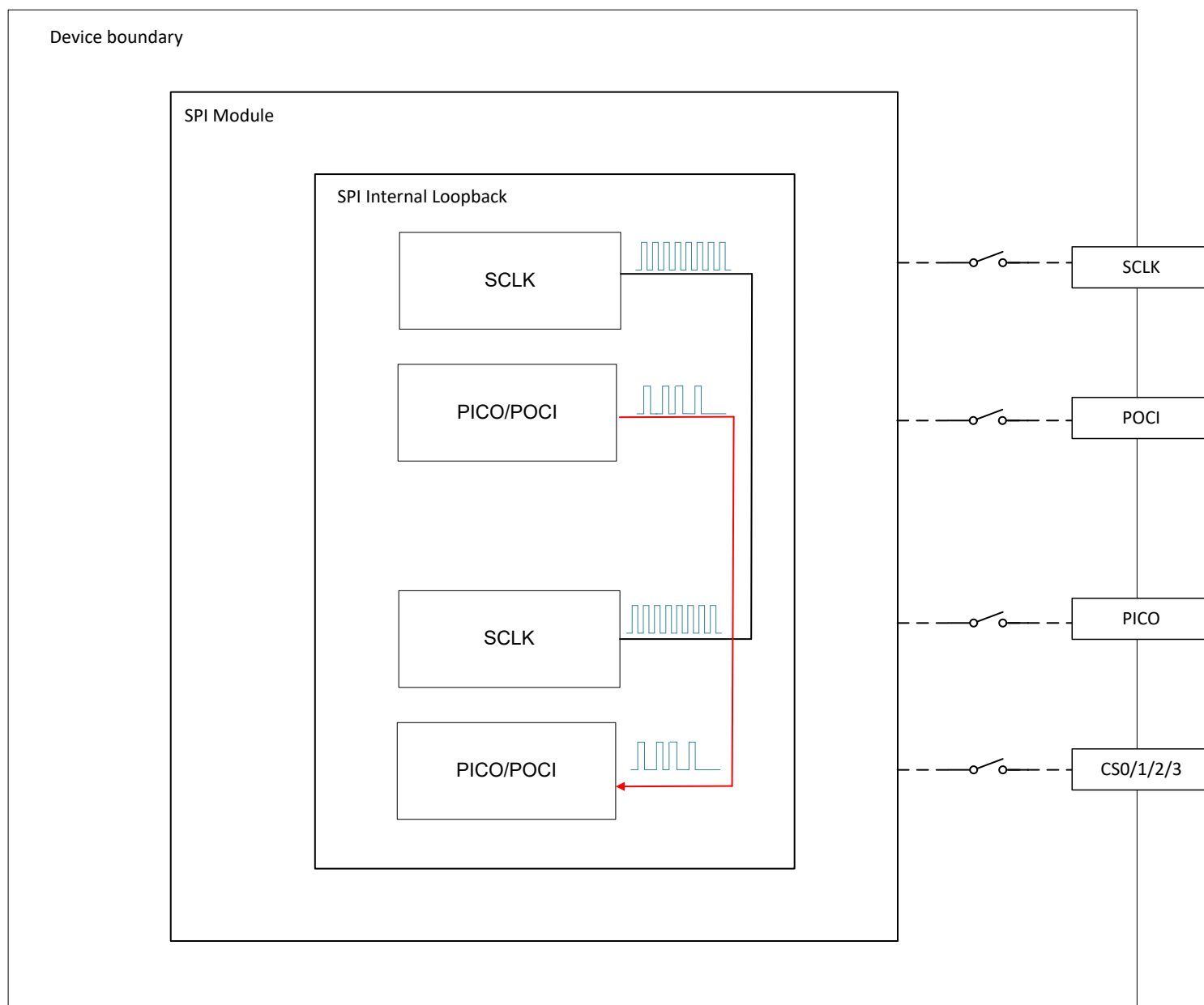
Figure 25-3. Internal Loop Back Mode
