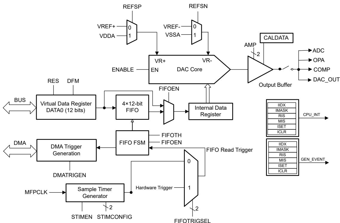
Figure 19-1. DAC Block Diagram
