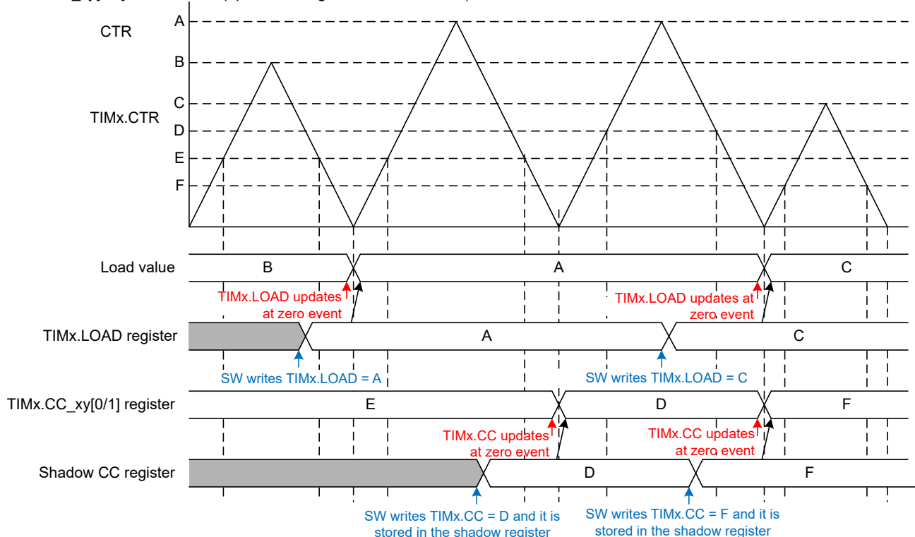
Figure 27-25. Shadow Load and Shadow Compare Taking Effect at Zero Event in Up/Down Mode
