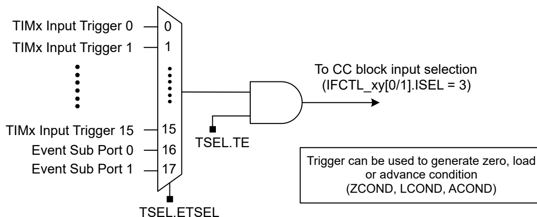
Figure 27-40. Secondary Timer Cross Trigger Input Configuration
