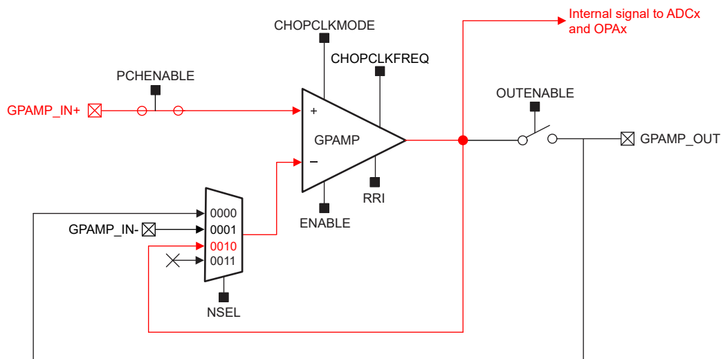
Figure 21-3. GPAMP in ADC Buffer Configuration
