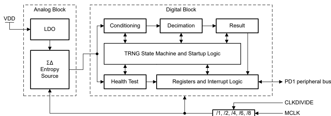
Figure 15-1. TRNG Block Diagram
