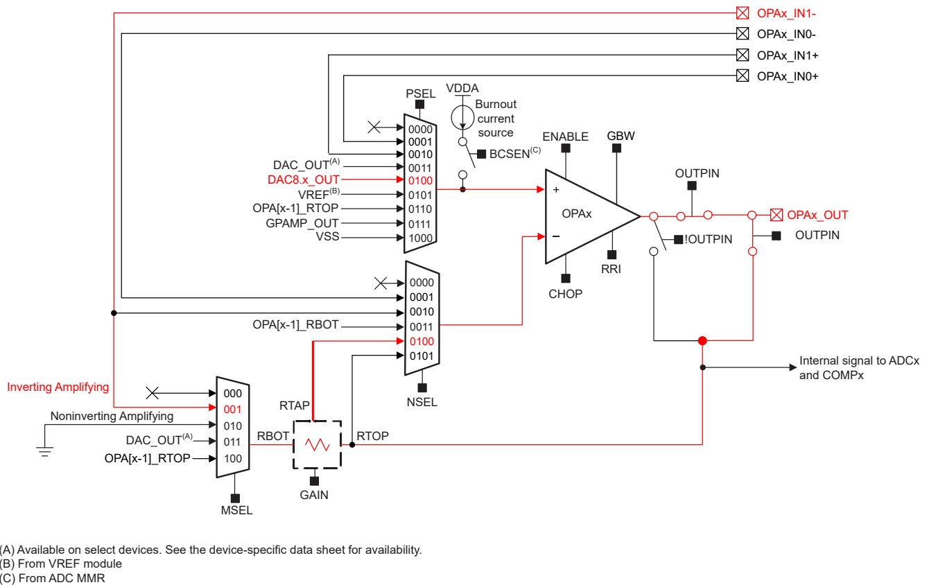
Figure 20-5. OPA in Inverting PGA Configuration
