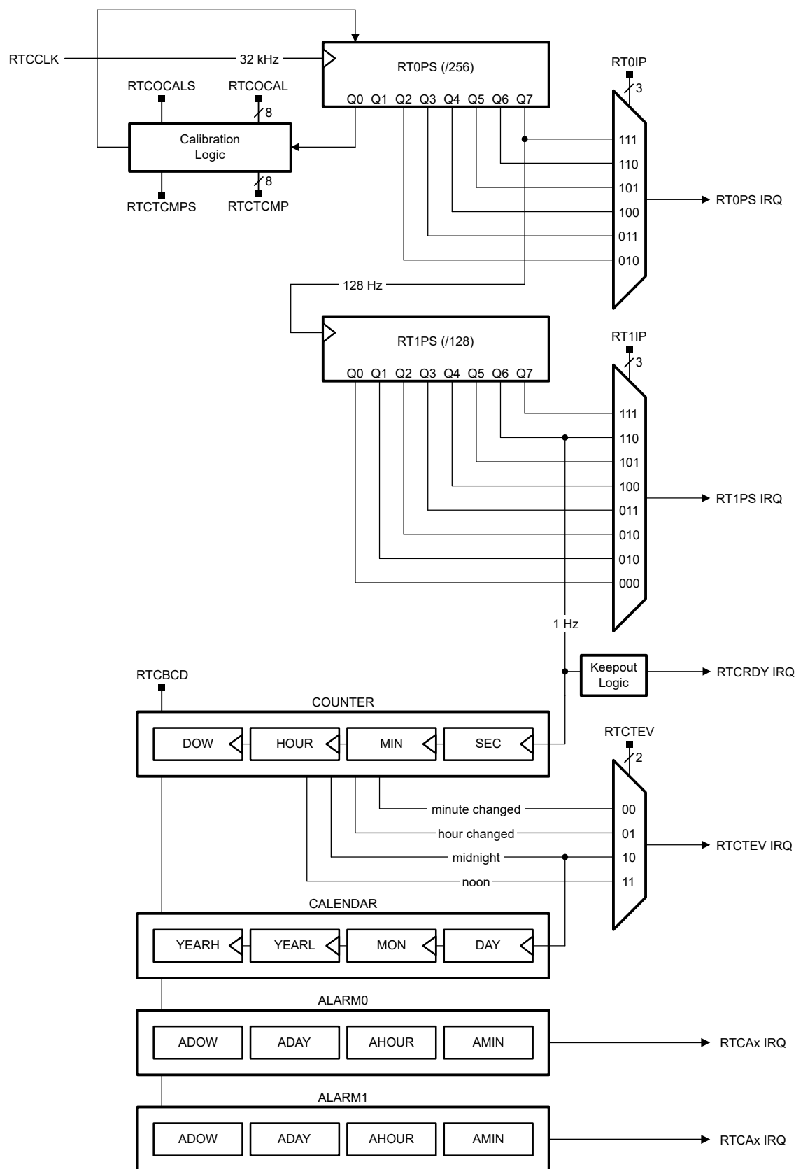
Figure 29-1. RTC Block Diagram
