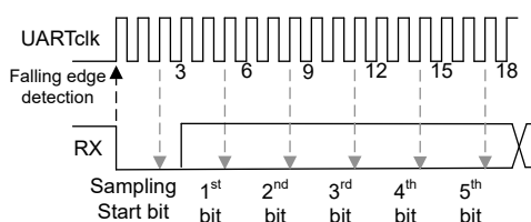
Figure 23-3. UART Oversampling mode
