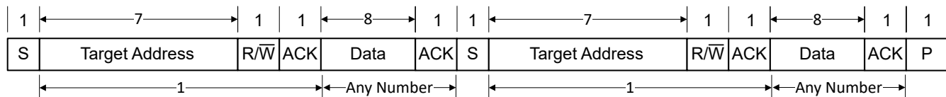
Figure 24-7. Data Format with Repeated Start
