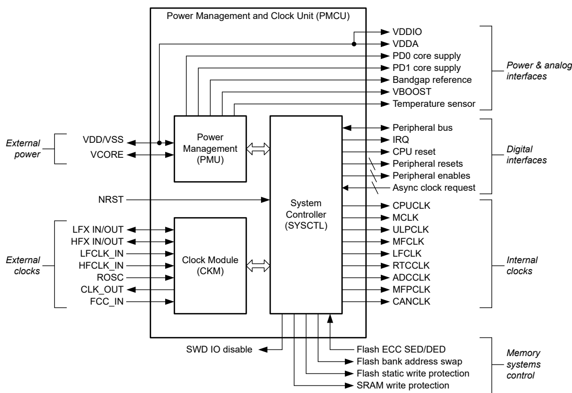
Figure 2-1. PMCU Top-Level Diagram
