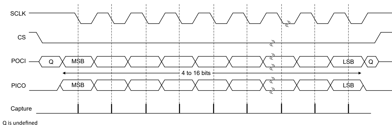
Figure 25-6. Motorola SPI Frame Format With SPO = 1 and SPH = 0
