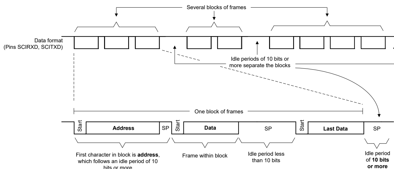
Figure 23-10. Idle-Line Multiprocessor
