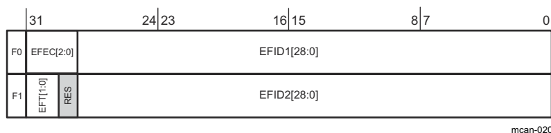
Figure 26-25. Extended Message ID Filter Element Structure
