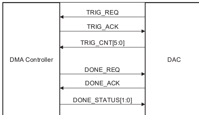
Figure 19-4. DAC Interface With DMA Controller
