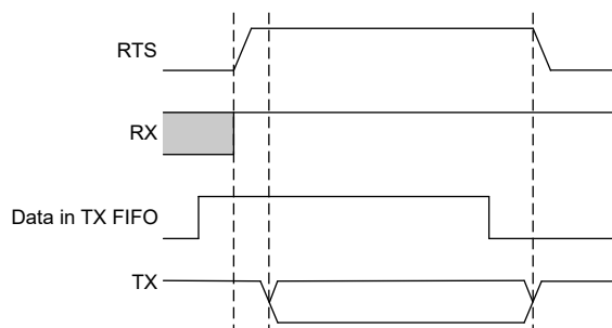
Figure 23-11. RS485 Data Exchange
