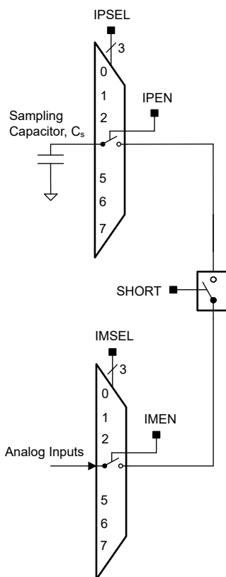
Figure 18-6. Comparator Short Switch
