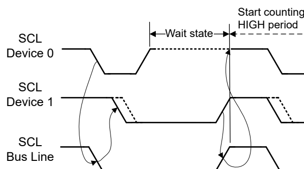
Figure 24-9. Clock Synchronization
