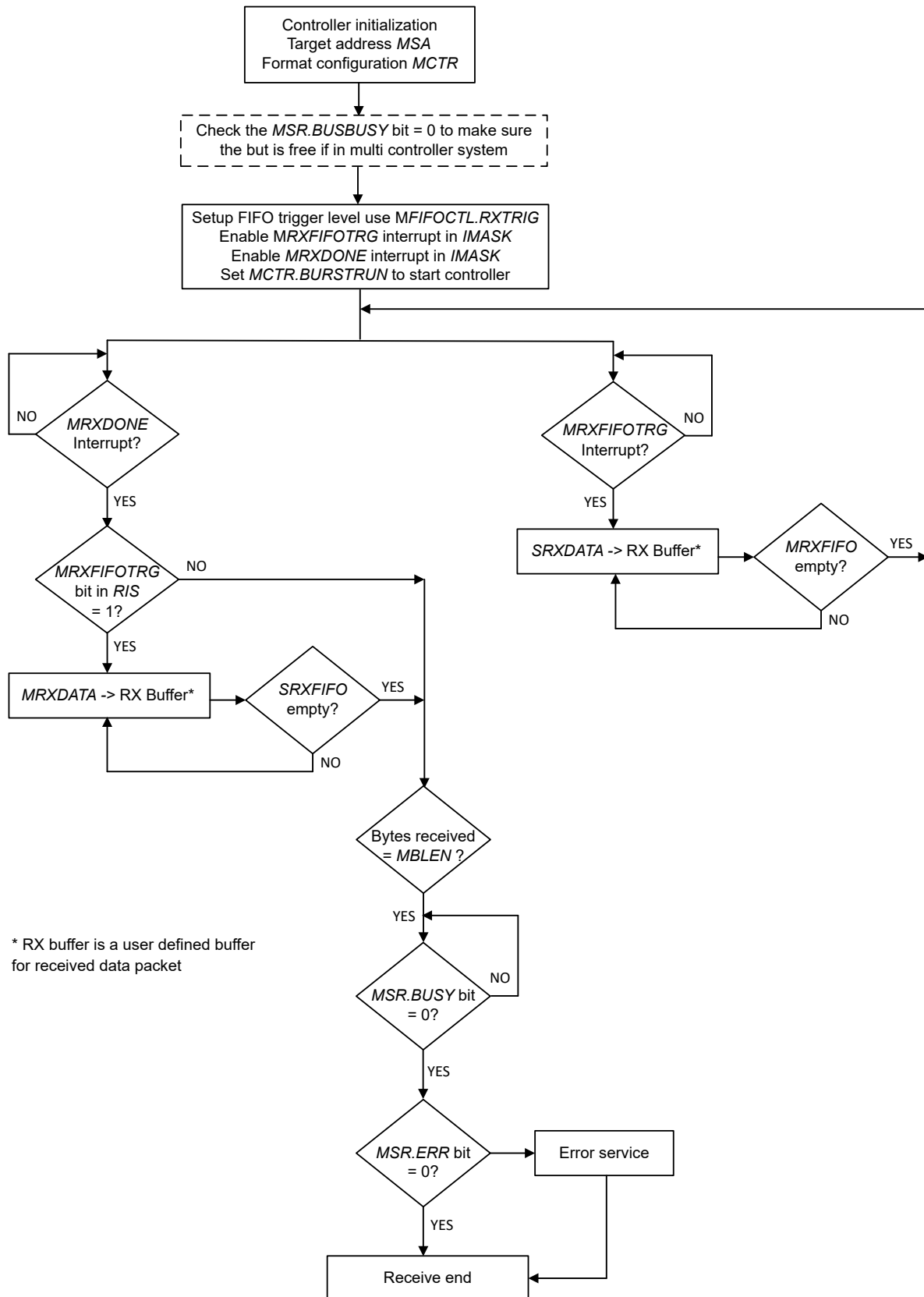
Figure 24-11. Controller Receiver Mode
