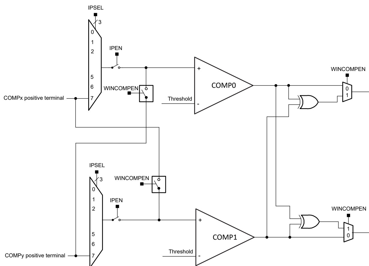
Figure 18-4. Window Comparator Mode
