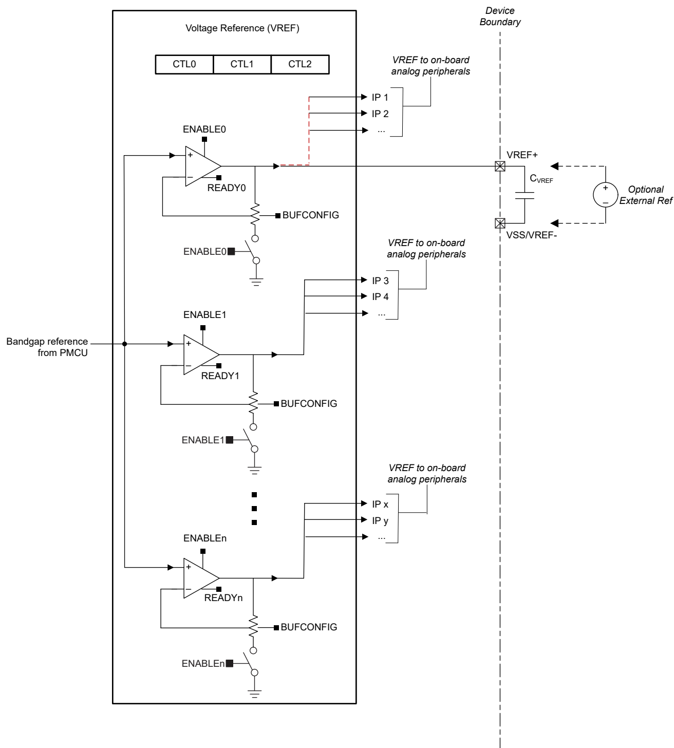
Figure 22-1. MSPM0 VREF Superset Block Diagram
