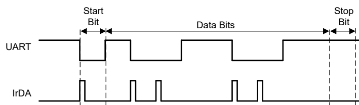
Figure 23-14. IrDA Protocol
