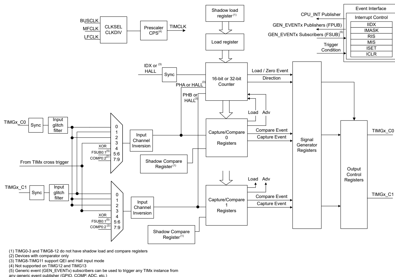
Figure 27-1. TIMx Functional Block Diagram
