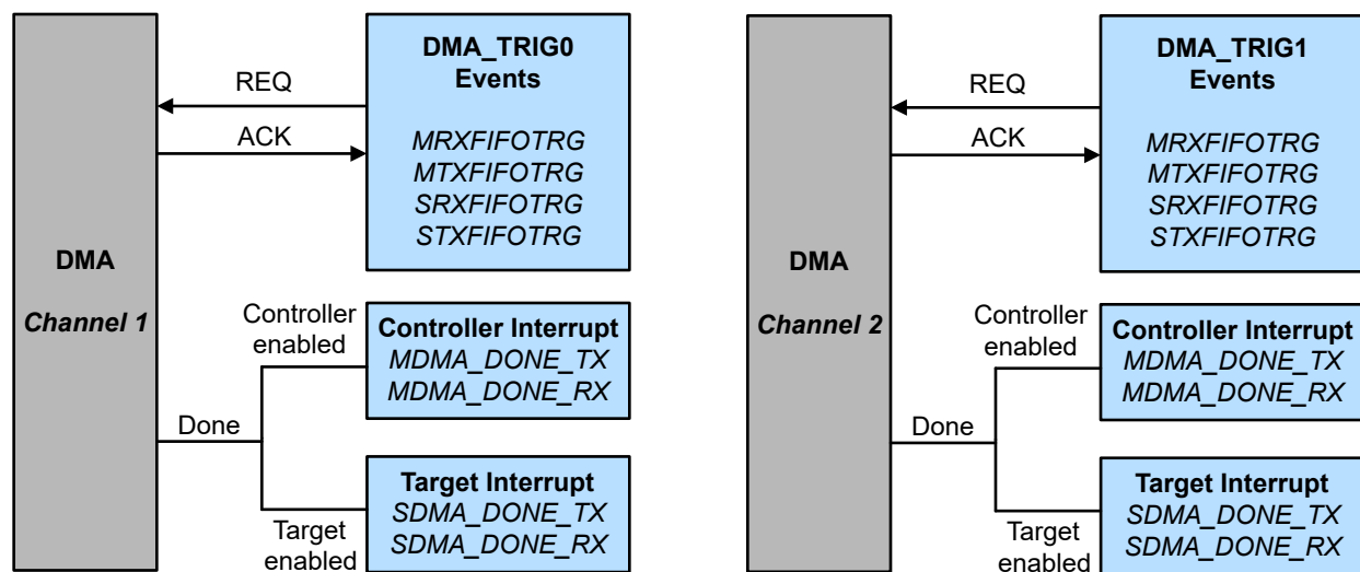
Figure 24-17. I 2 C DMA Trigger and Status
