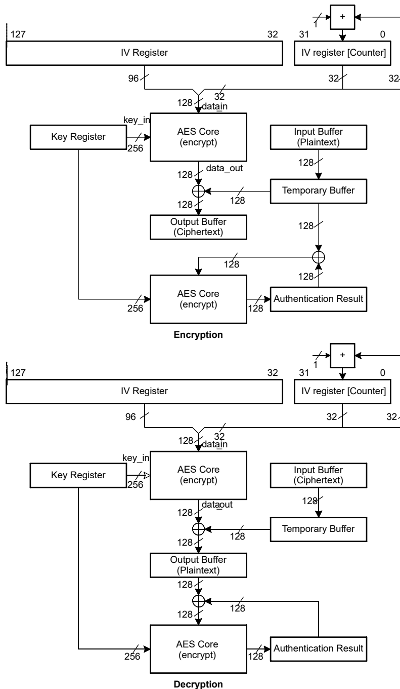
Figure 12-10. CCM Operation
