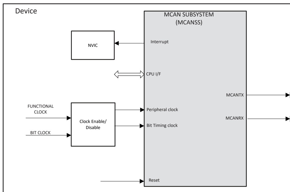
Figure 26-1. MCAN Block Diagram
