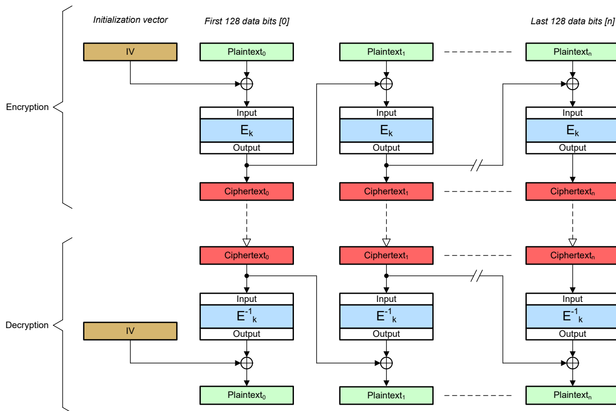
Figure 11-6. CBC Cipher
