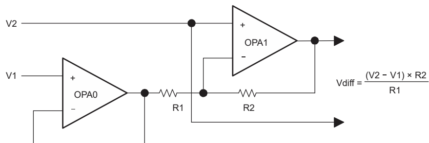
Figure 20-7. Two OPA Difference Amplifier Block Diagram and Equation
