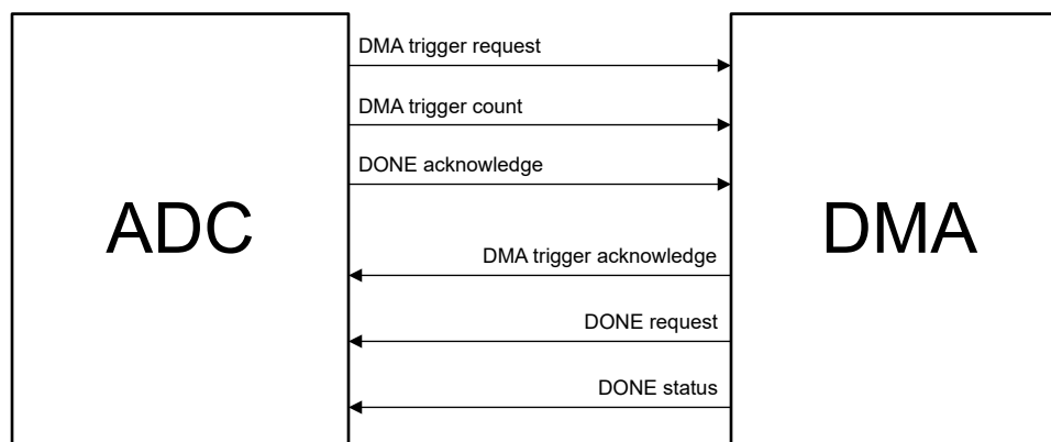
Figure 17-4. Internal ADC-DMA Interface
