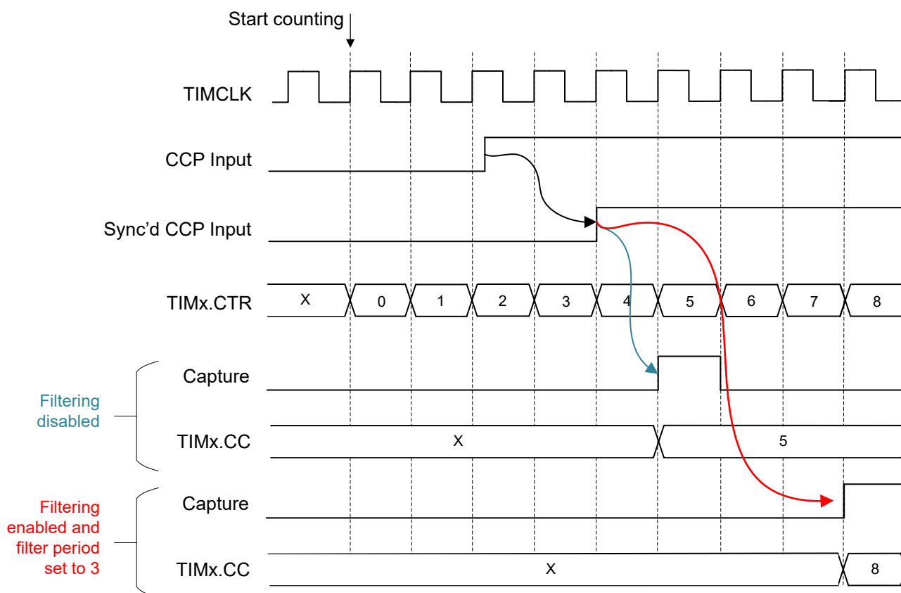
Figure 27-14. Edge Time Capture Mode in Up-Counting Mode, CVAE = 2
