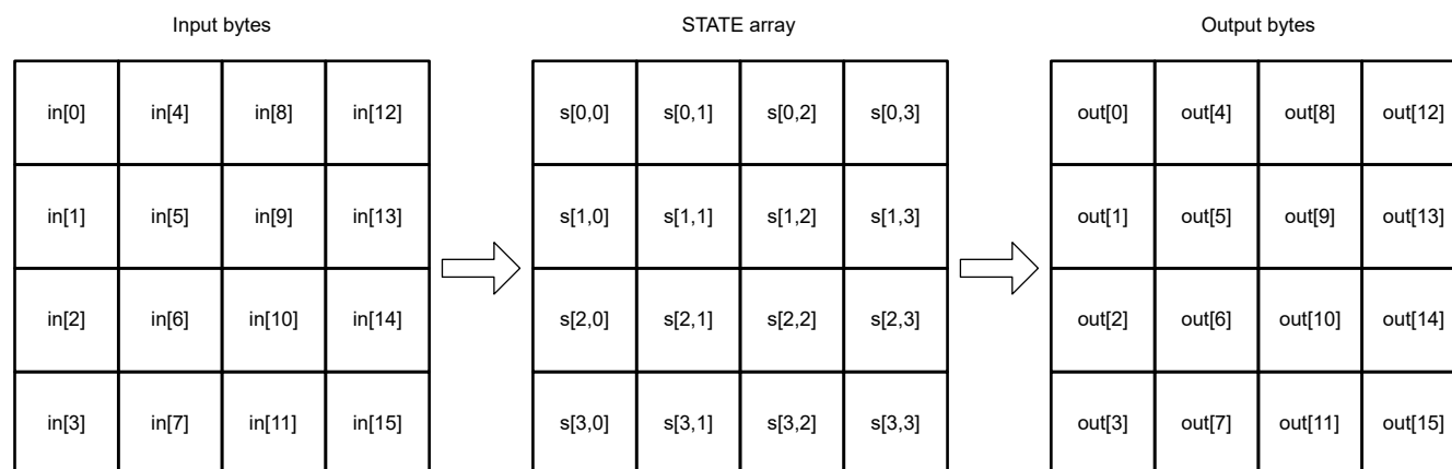
Figure 11-2. AES State Array Input and Output
