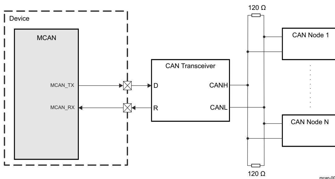
Figure 26-2. MCAN Typical Bus Wiring
