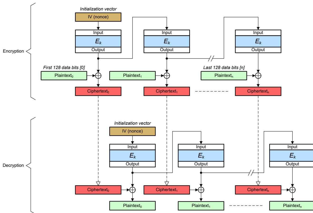
Figure 12-4. OFB Cipher
