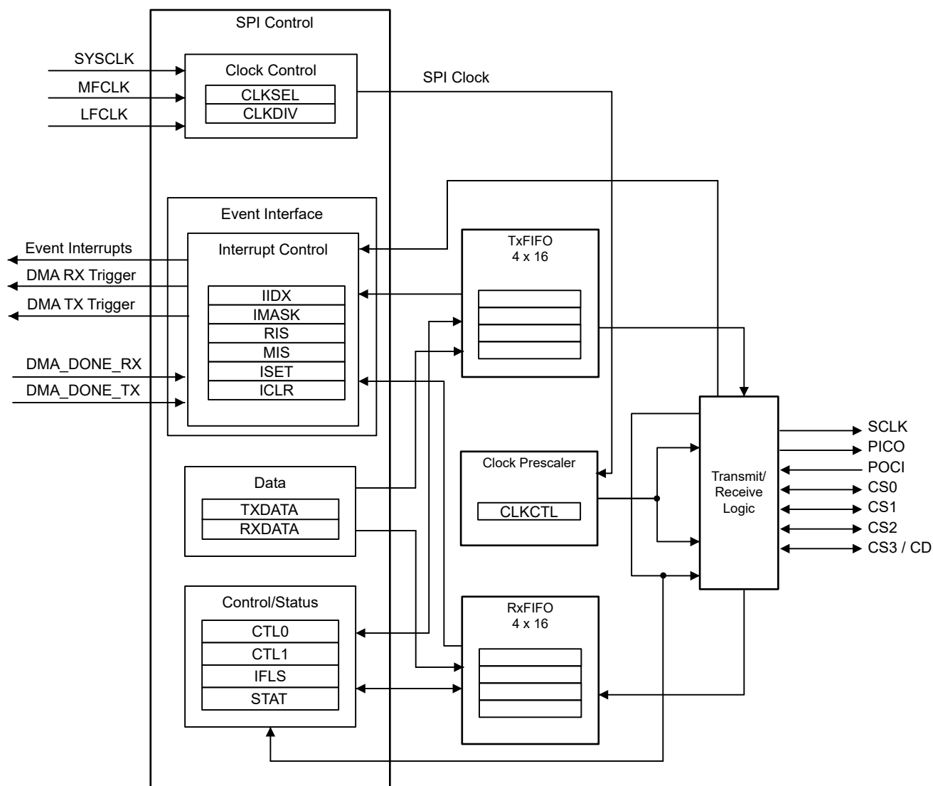
Figure 25-1. SPI Functional Block Diagram
