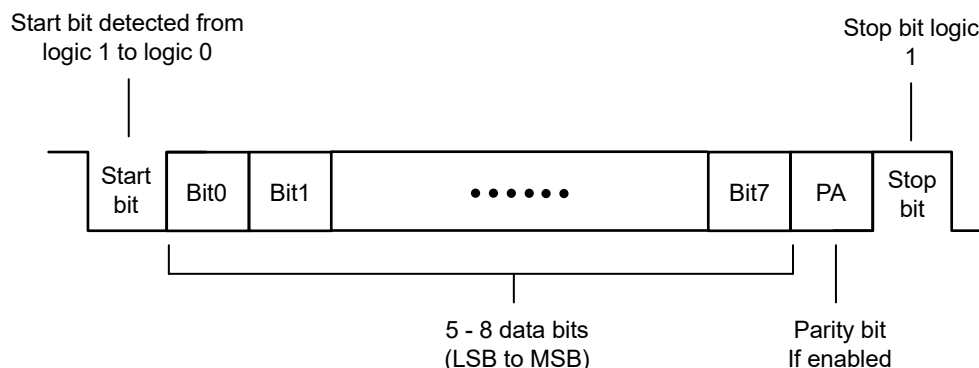
Figure 23-2. UART Character Frame
