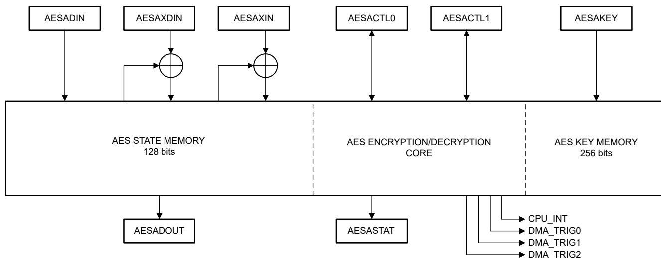
Figure 11-1. AES Accelerator Block Diagram
