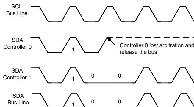
Figure 24-8. Arbitration Procedure Between Two Controller Transmitters
