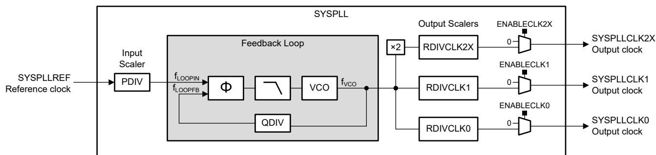
Figure 2-7. SYSPLL Diagram
