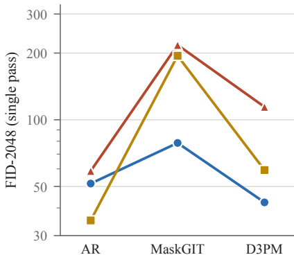
(b) FID-2048, same generated samples
