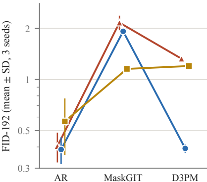
(a) FID-192, three training seeds
