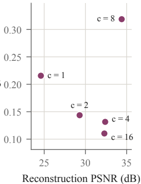
(b) VAE channels, \rho = +0.10
