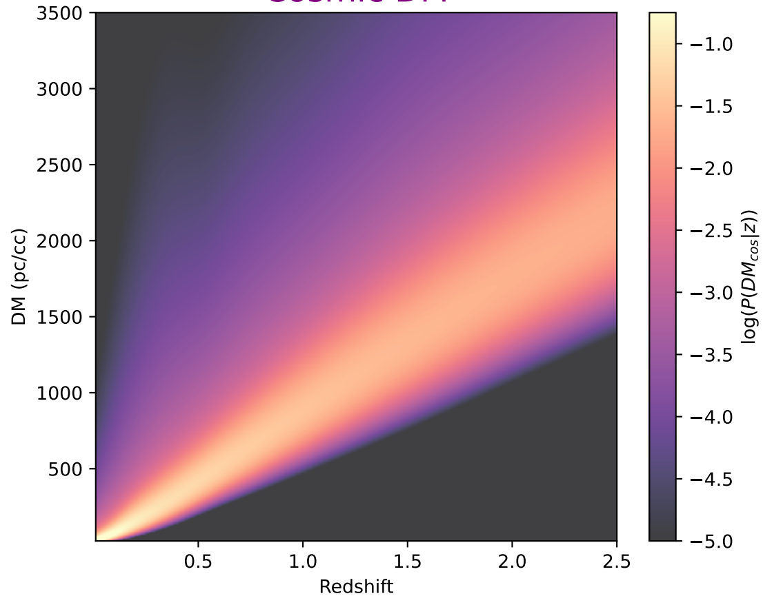
Cosmic DM
