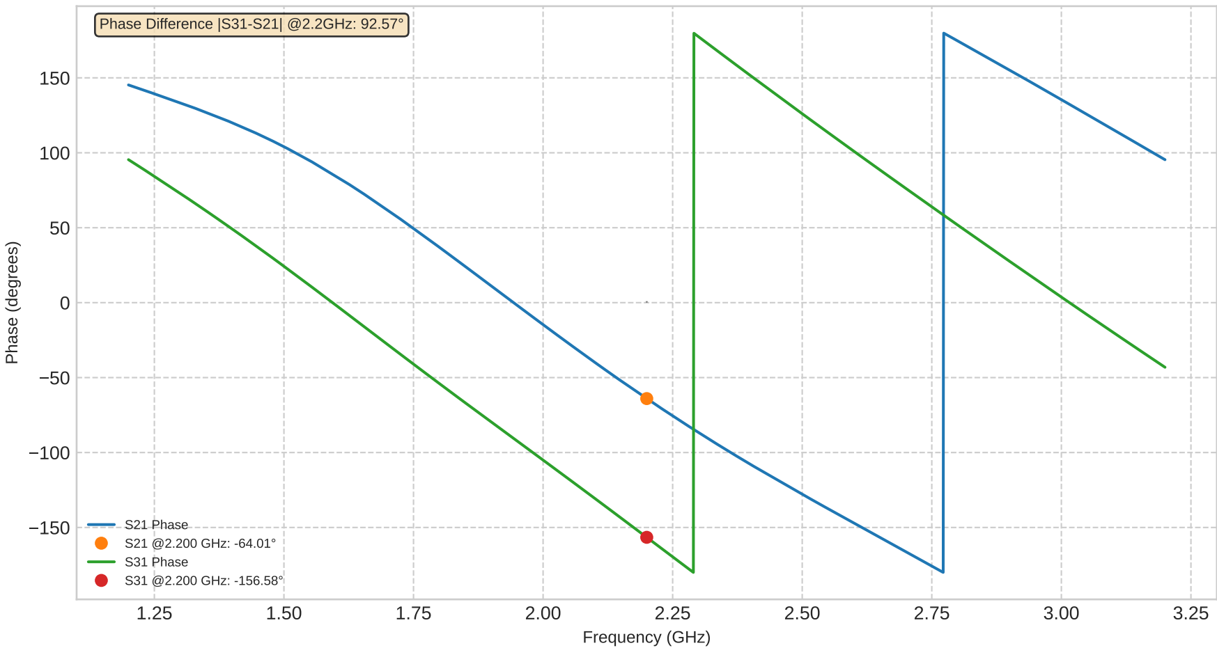
VNA Measurement: S-Parameter Phases - Coupler V2
