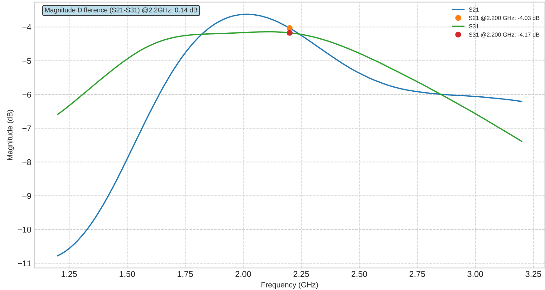
VNA Measurement: S-Parameter Magnitudes - Coupler V2
