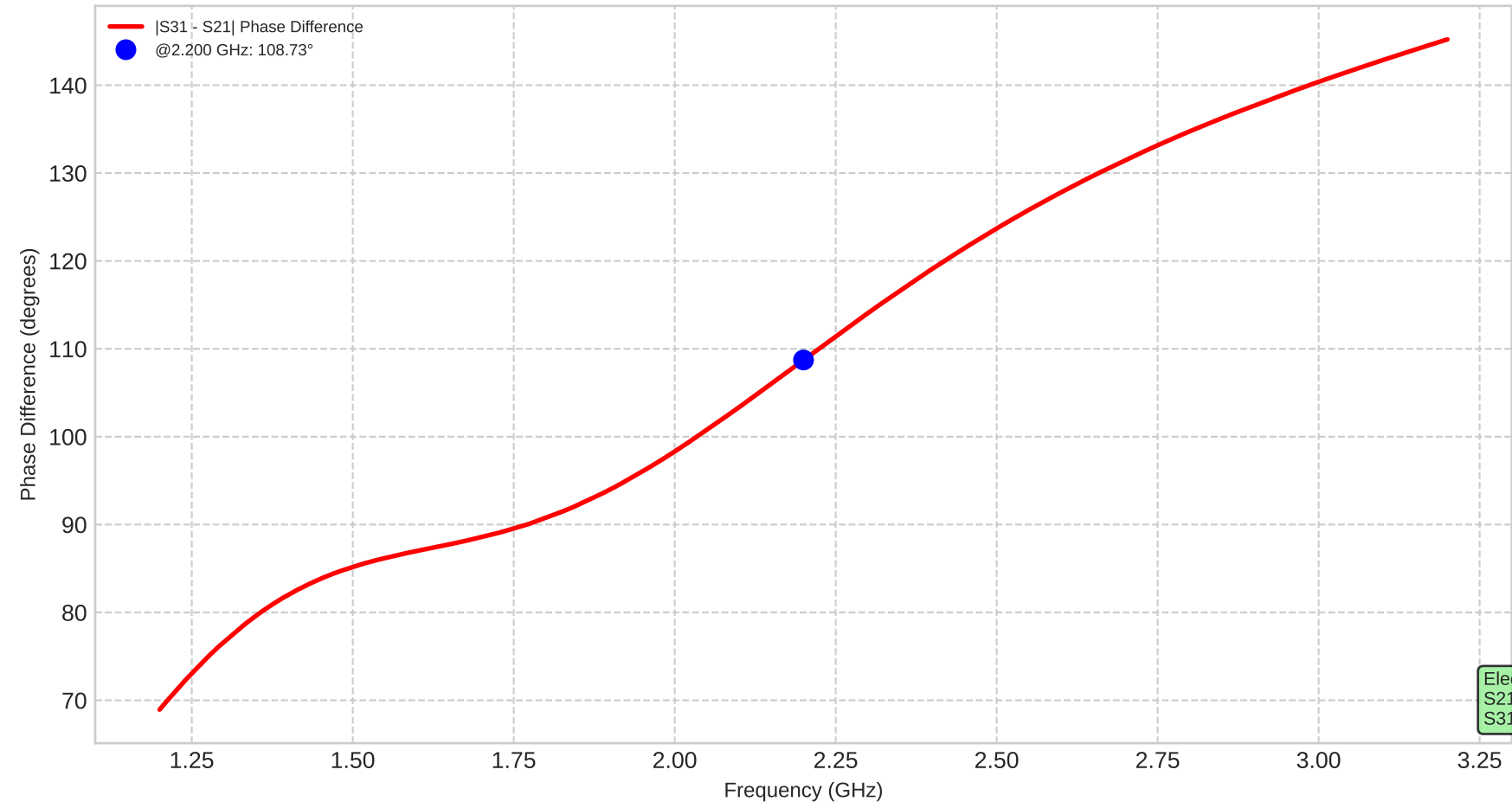
VNA Measurement: Phase Difference |S31 - S21| - Coupler V1
