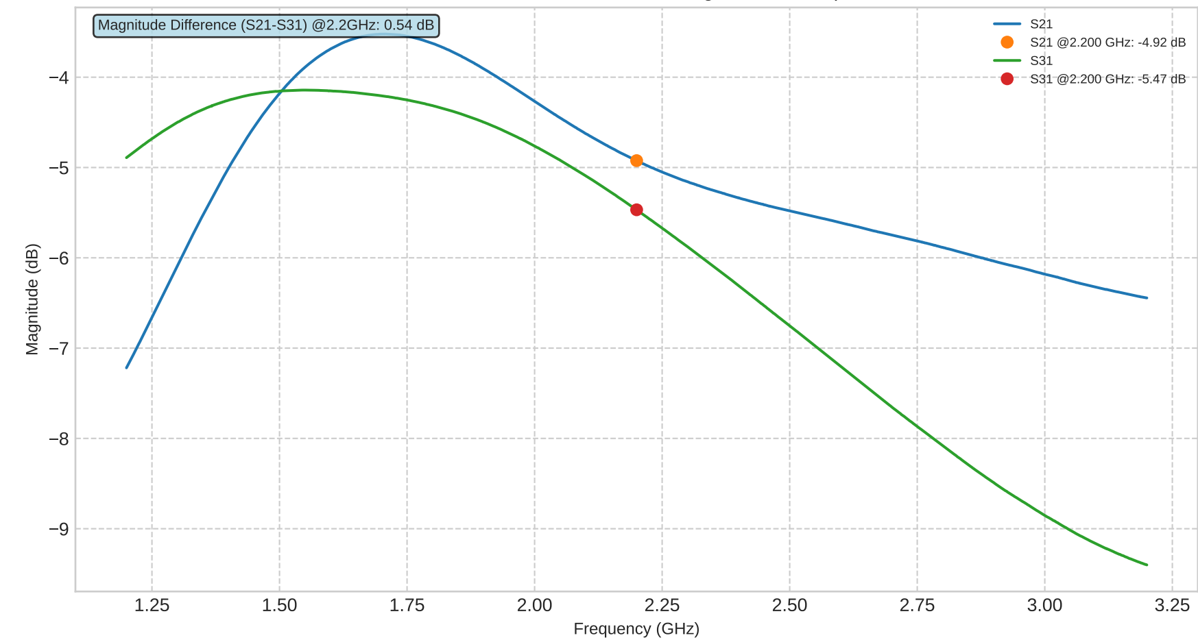
VNA Measurement: S-Parameter Magnitudes - Coupler V1
