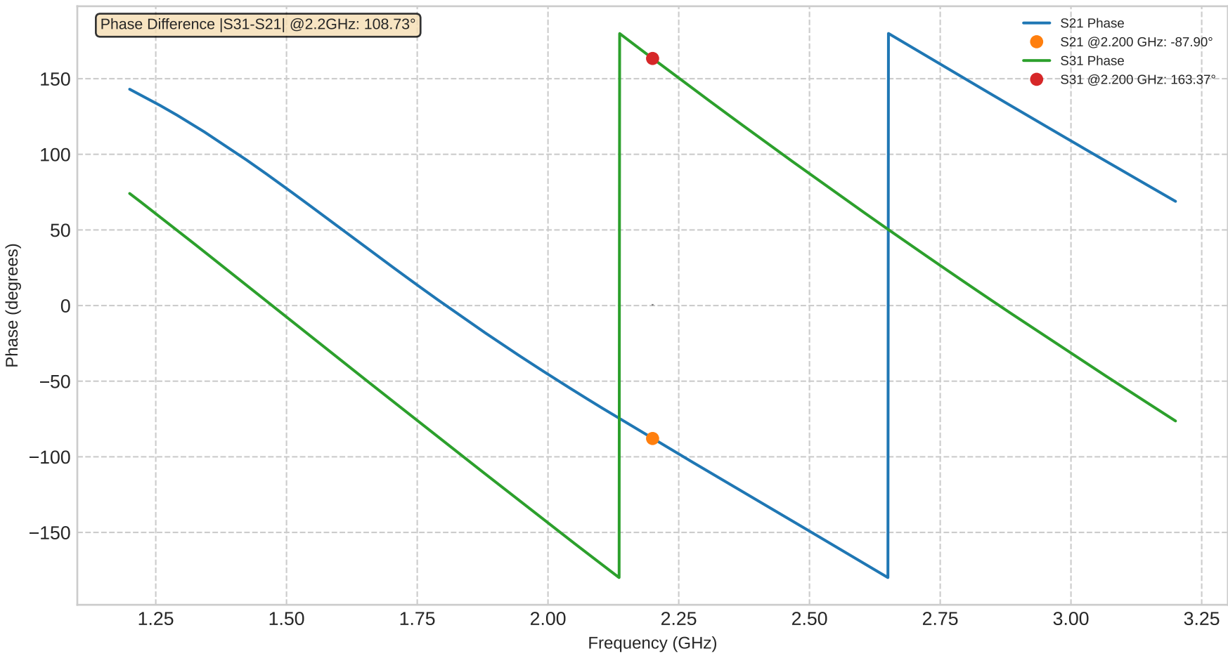
VNA Measurement: S-Parameter Phases - Coupler V1
