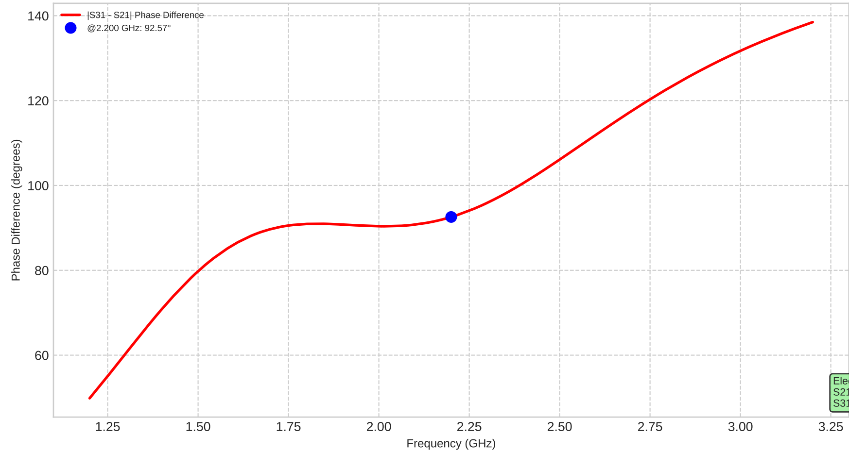
VNA Measurement: Phase Difference |S31 - S21| - Coupler V2
