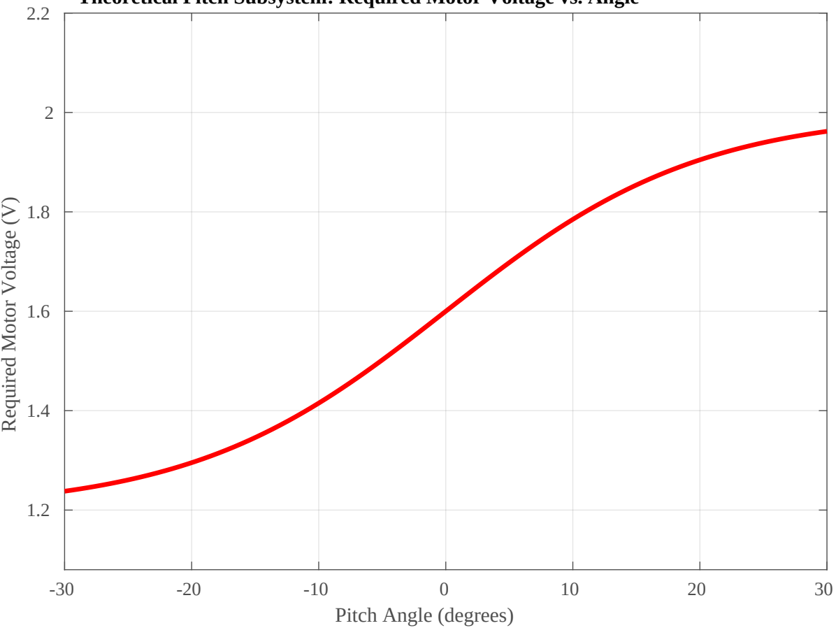
Theoretical Pitch Subsystem: Required Motor Voltage vs. Angle
