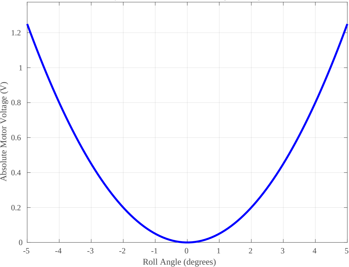
Theoretical Roll Subsystem: Absolute Motor Voltage vs. Angle
