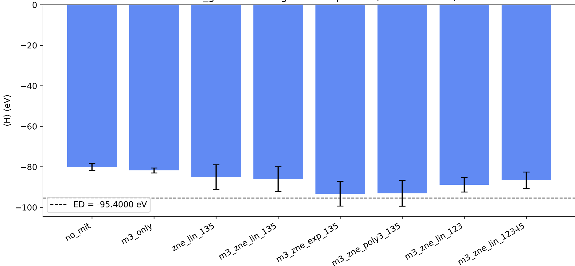
L2 NiO e_g^2 SIAM — mitigation comparison (FakeMarrakesh)
