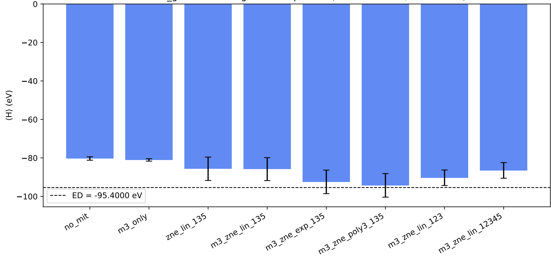
L2 NiO e_g^2 SIAM — mitigation comparison (FakeMarrakesh, 8192 shots)
