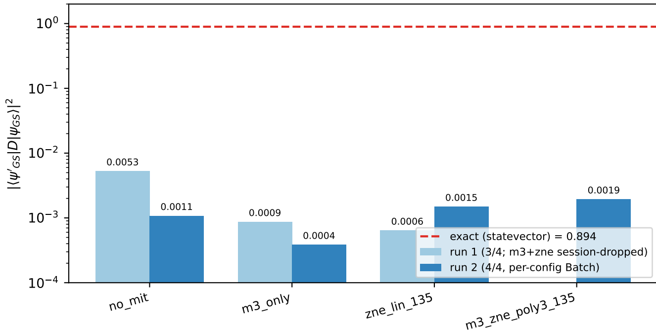
L1 cross-sector dipole matrix element on ibm_marrakesh (all configs collapse \sim 0.89 \rightarrow \sim 0.001 ; mitigation does not recover)
