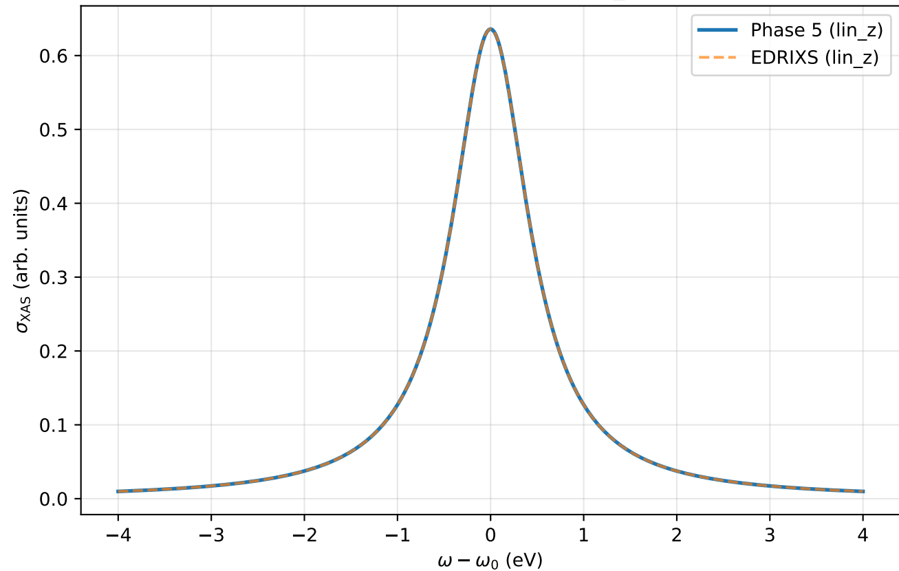
L-edge XAS - channel lin_z
