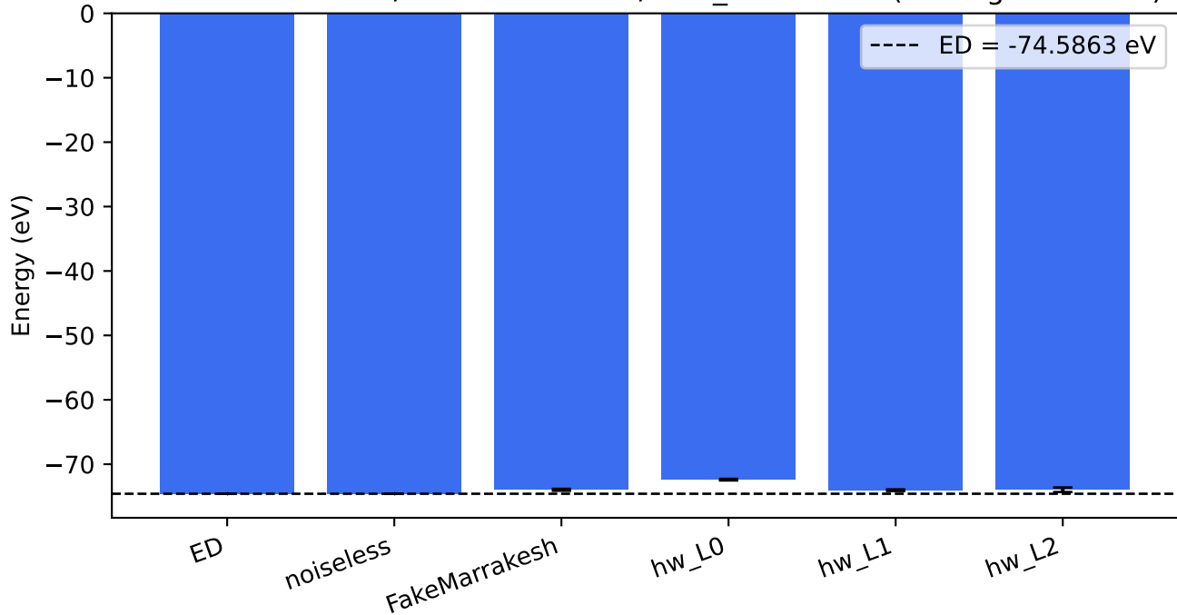
L1 NiO SIAM — noiseless / FakeMarrakesh / ibm_marrakesh (3 mitigation tiers) vs
