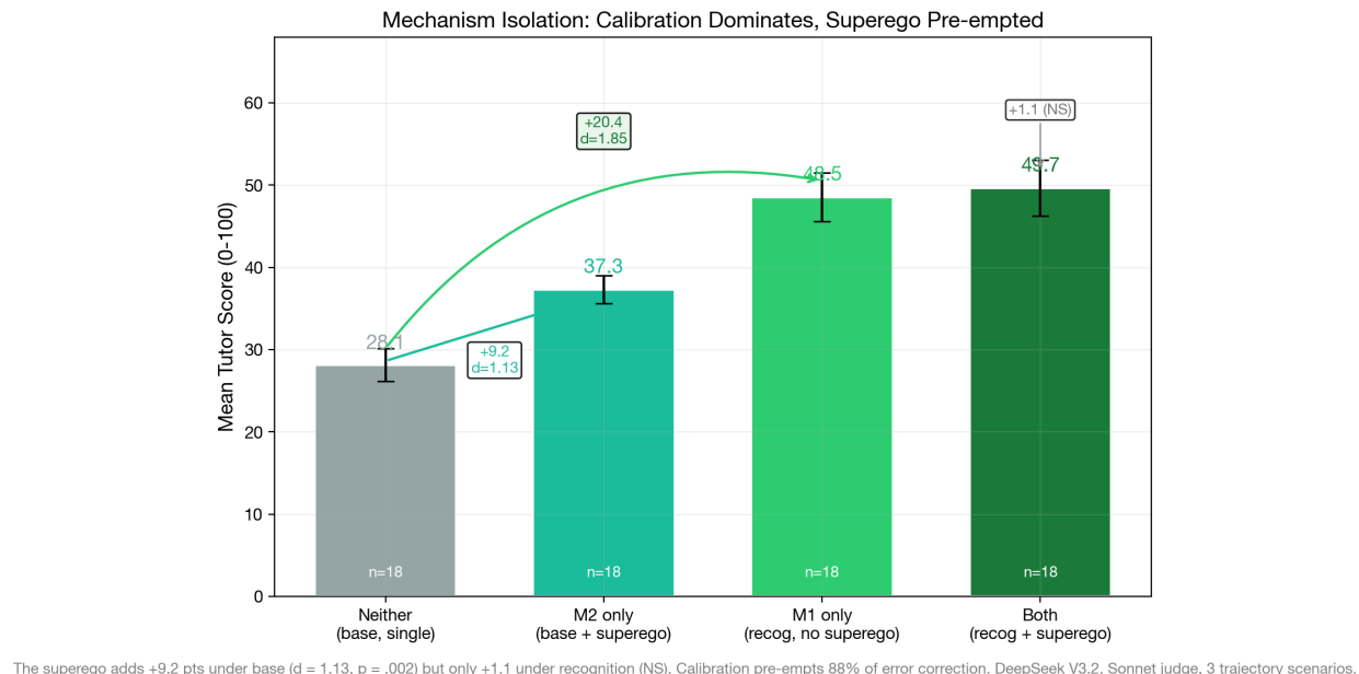
Figure 3: Mechanism isolation: the superego adds +9.2 pts under base ( d=1.13 ) but only +1.1 under recognition (NS). Calibration alone (M1, d=1.85 from baseline) accounts for most of the total effect; adding the superego when calibration is present yields negligible gain. DeepSeek V3.2, Sonnet judge, 3 trajectory scenarios, N=72 .
