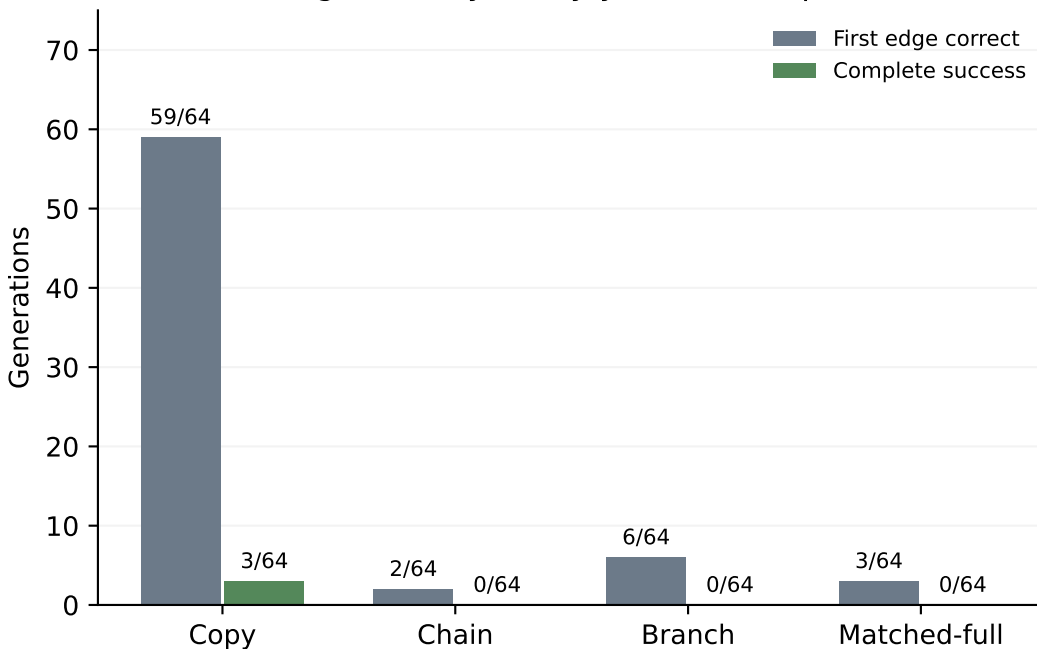
A Starting correctly rarely yields a complete route
