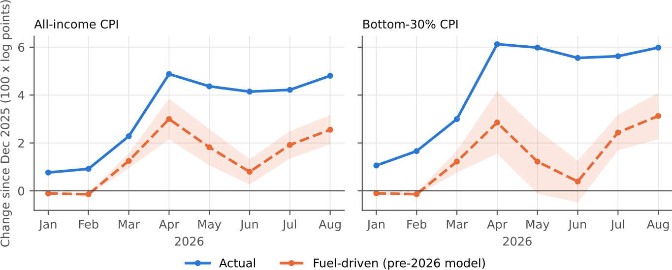
Figure 6. The 2026 shock: actual price rise vs. fuel-driven rise predicted by a model estimated only on 2001-2025 data
