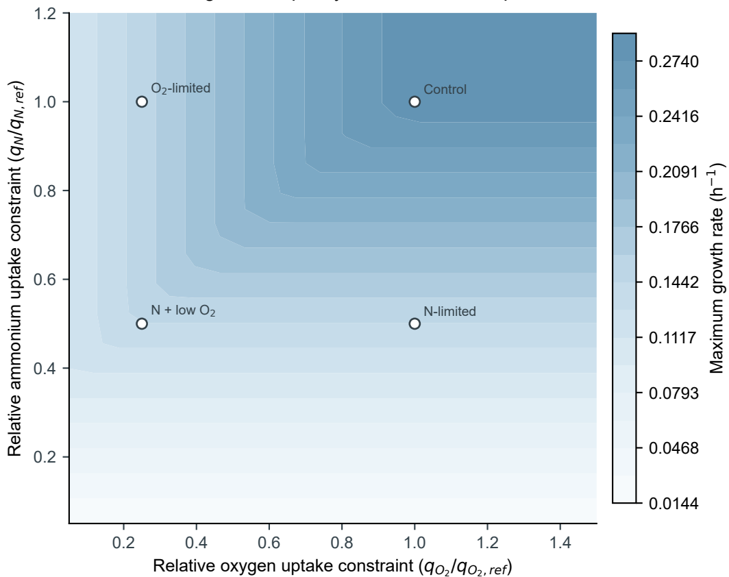
Maximum growth capacity across the N-O 2 plane
