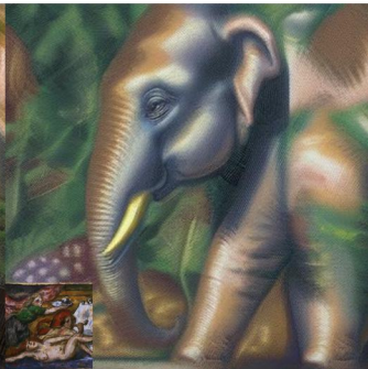
V1 adain_1blk
