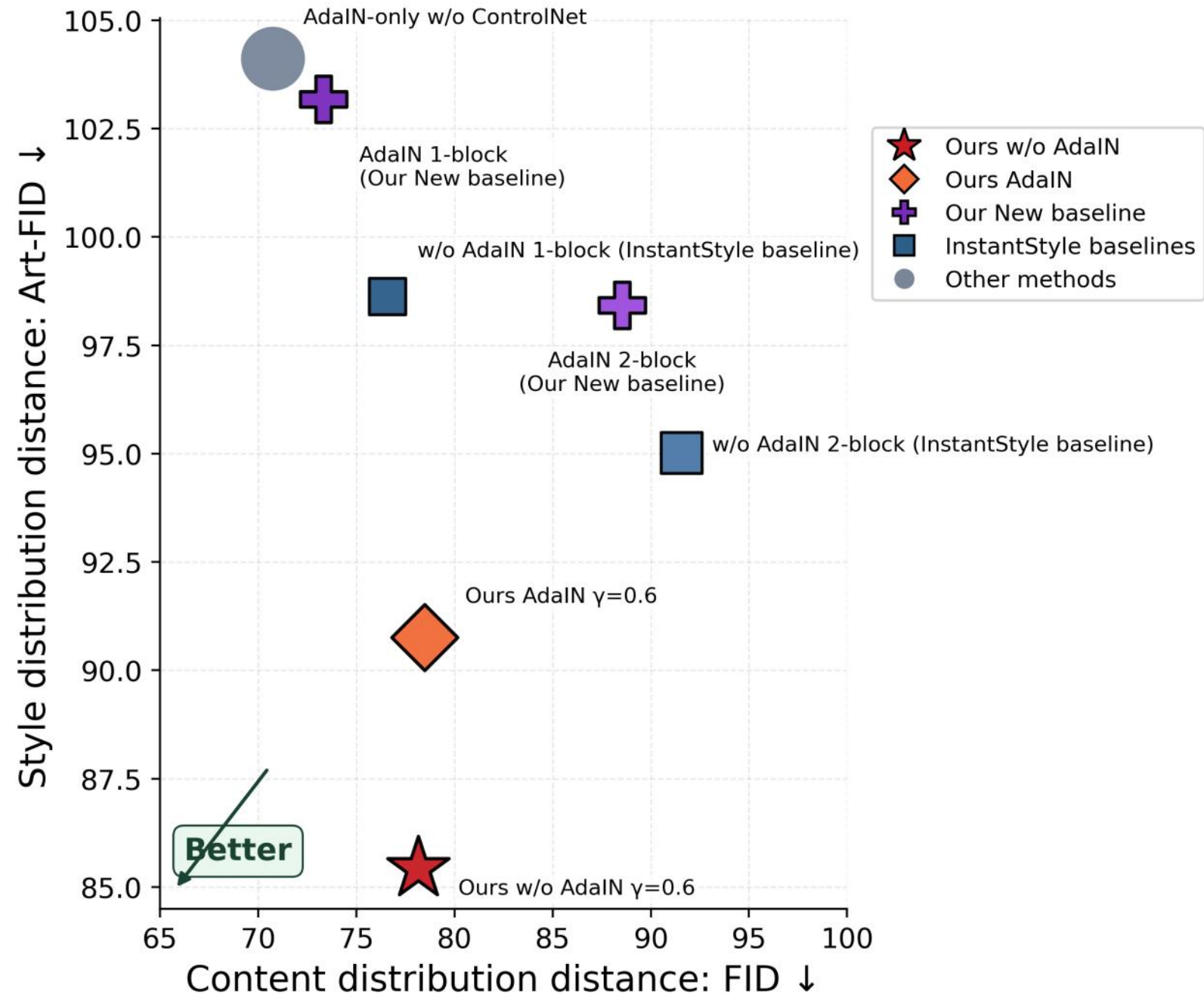
Content-Style Trade-off on 5k Evaluation Set
