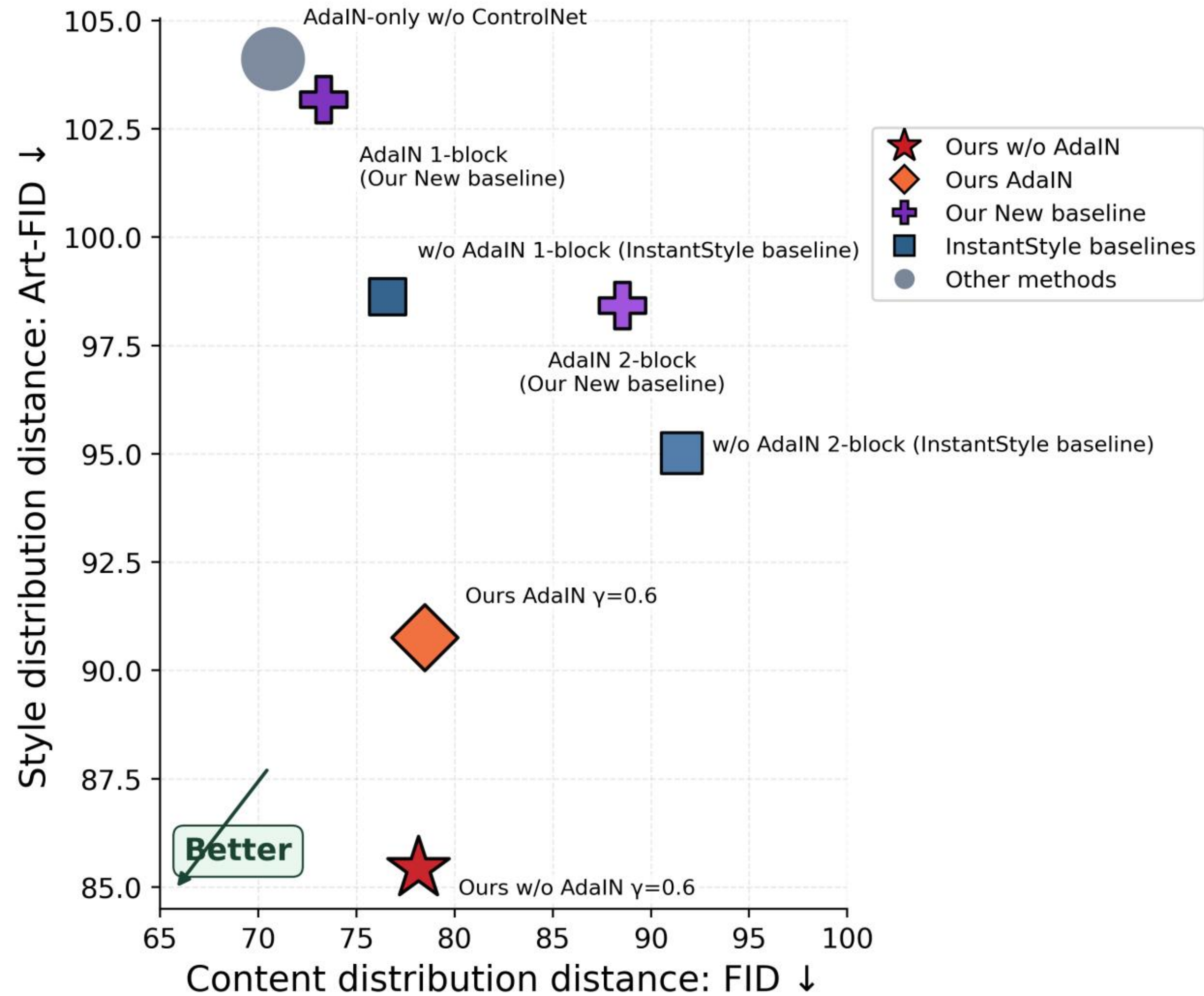
Content-Style Trade-off on 5k Evaluation Set
