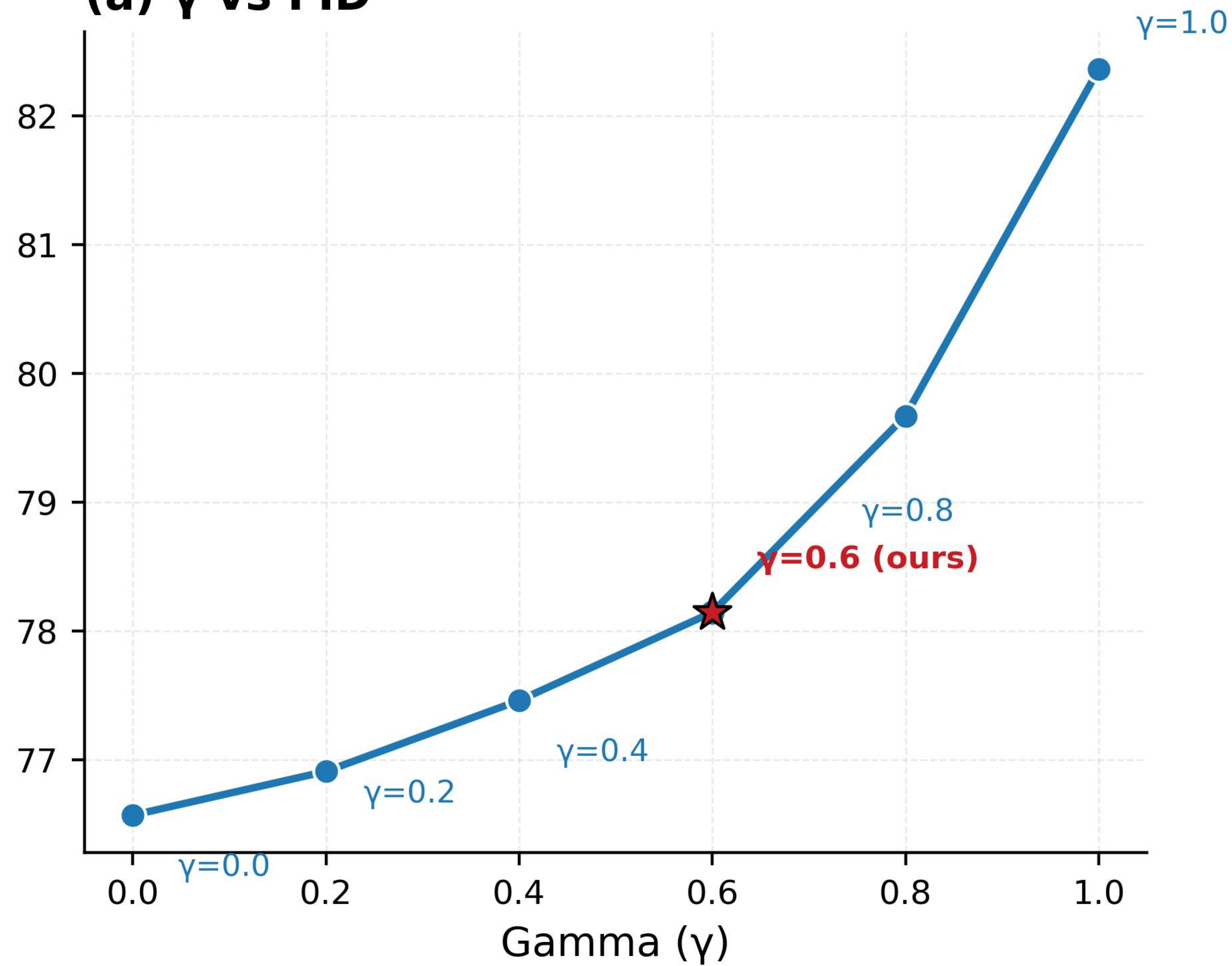
(a) \gamma vs FID
