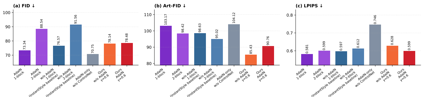
Fig. 6. Quantitative comparison of 7 method variants across FID, Art-FID, and LPIPS metrics (lower is better for all three). FID reflects distribution distance from the content domain, Art-FID reflects proximity to the target artistic style domain, and LPIPS reflects the perceptual-level image change magnitude. V6 (Ours w/o AdaIN) achieves the lowest Art-FID, indicating stronger style injection; compared with V6, the full method V7 (Ours AdaIN, \gamma = 0.6 ) reduces LPIPS, indicating milder perceptual change.
