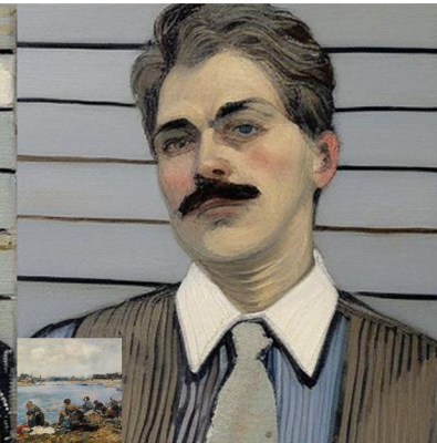
adain_2blk
